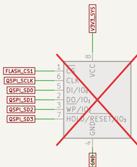
U24 DNP: W25Q64JVSSIQ, 64 Mbit QSPI NOR (optional back-side expansion)
