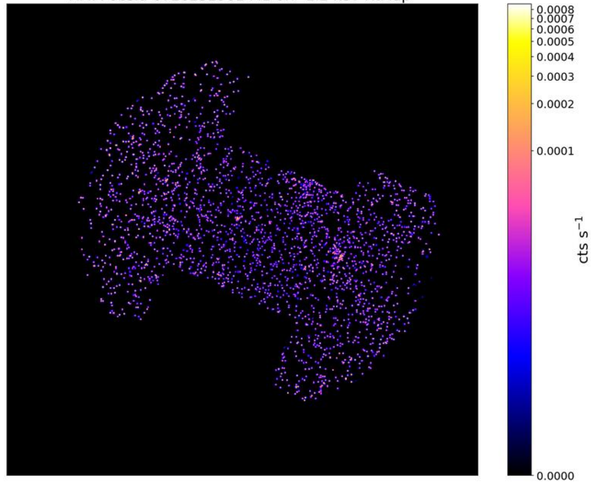
LoVoCCS-106-SH518: \text{Exp}_{\text{clean}}/\text{Exp}_{\text{tot}} = 0.30 XMM obsid-0720252901 M1 0.7-1.2 keV RtMap
