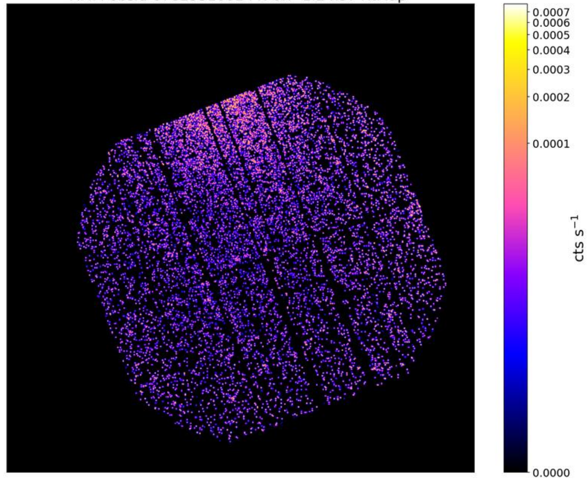
LoVoCCS-117-A2063: \text{Exp}_{\text{clean}}/\text{Exp}_{\text{tot}} = 0.64 XMM obsid-0782531001 PN 0.7-1.2 keV RtMap
