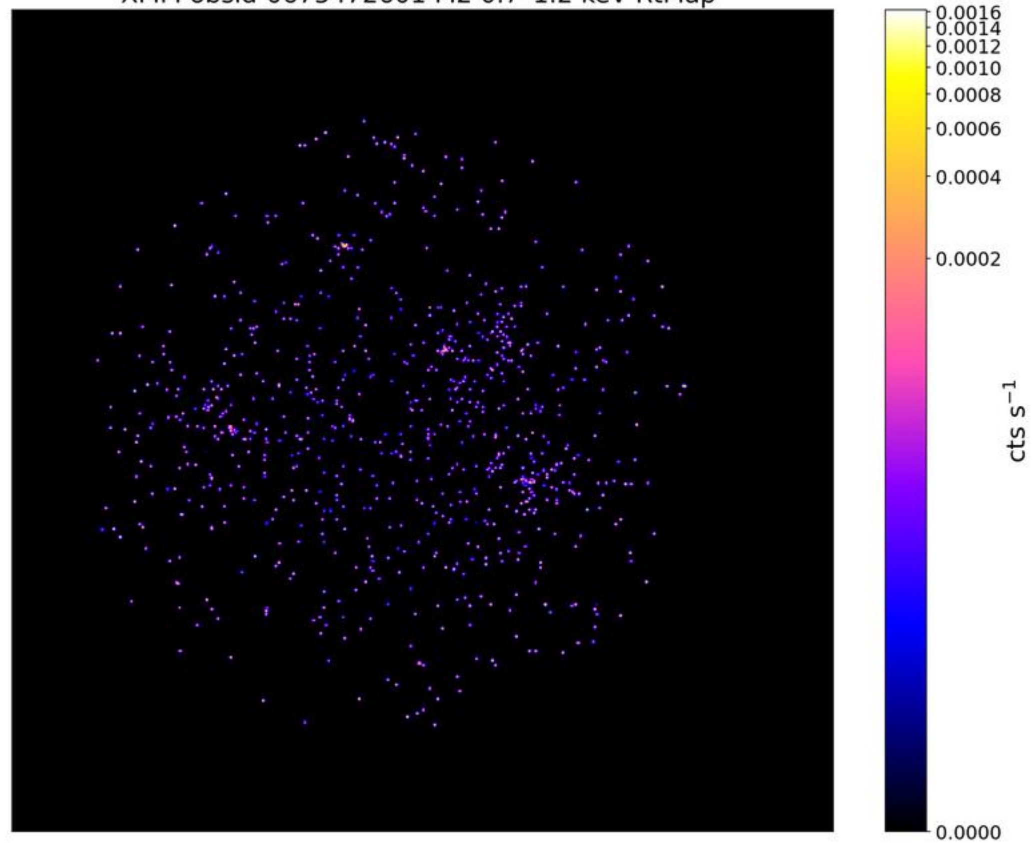
LoVoCCS-103-MCXJ0034.6-0208: \text{Exp}_{\text{clean}}/\text{Exp}_{\text{tot}} = 0.19 XMM obsid-0675472601 M2 0.7-1.2 keV RtMap
