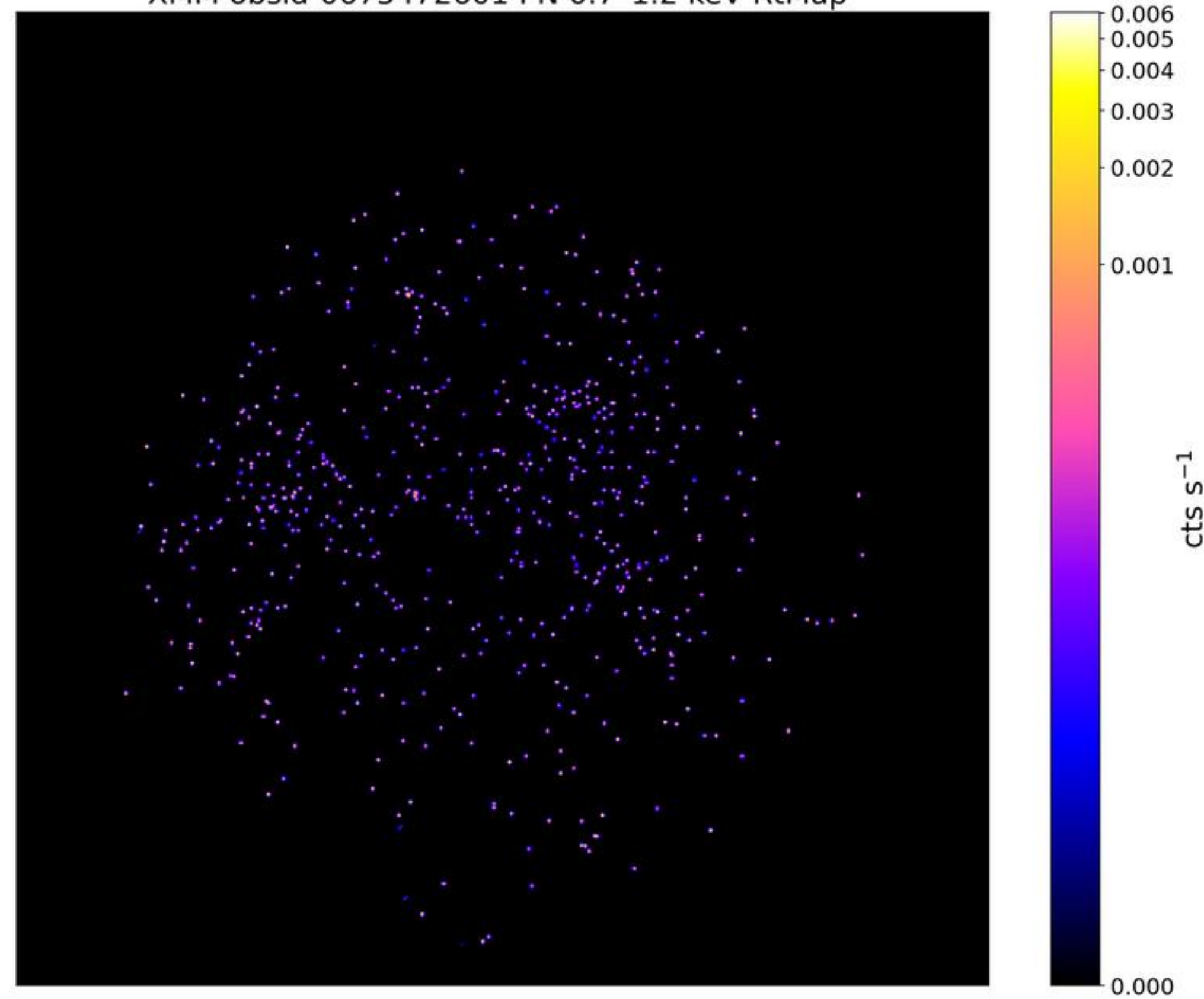
LoVoCCS-103-MCXJ0034.6-0208: \text{Exp}_{\text{clean}}/\text{Exp}_{\text{tot}} = 0.03 XMM obsid-0675472601 PN 0.7-1.2 keV RtMap
