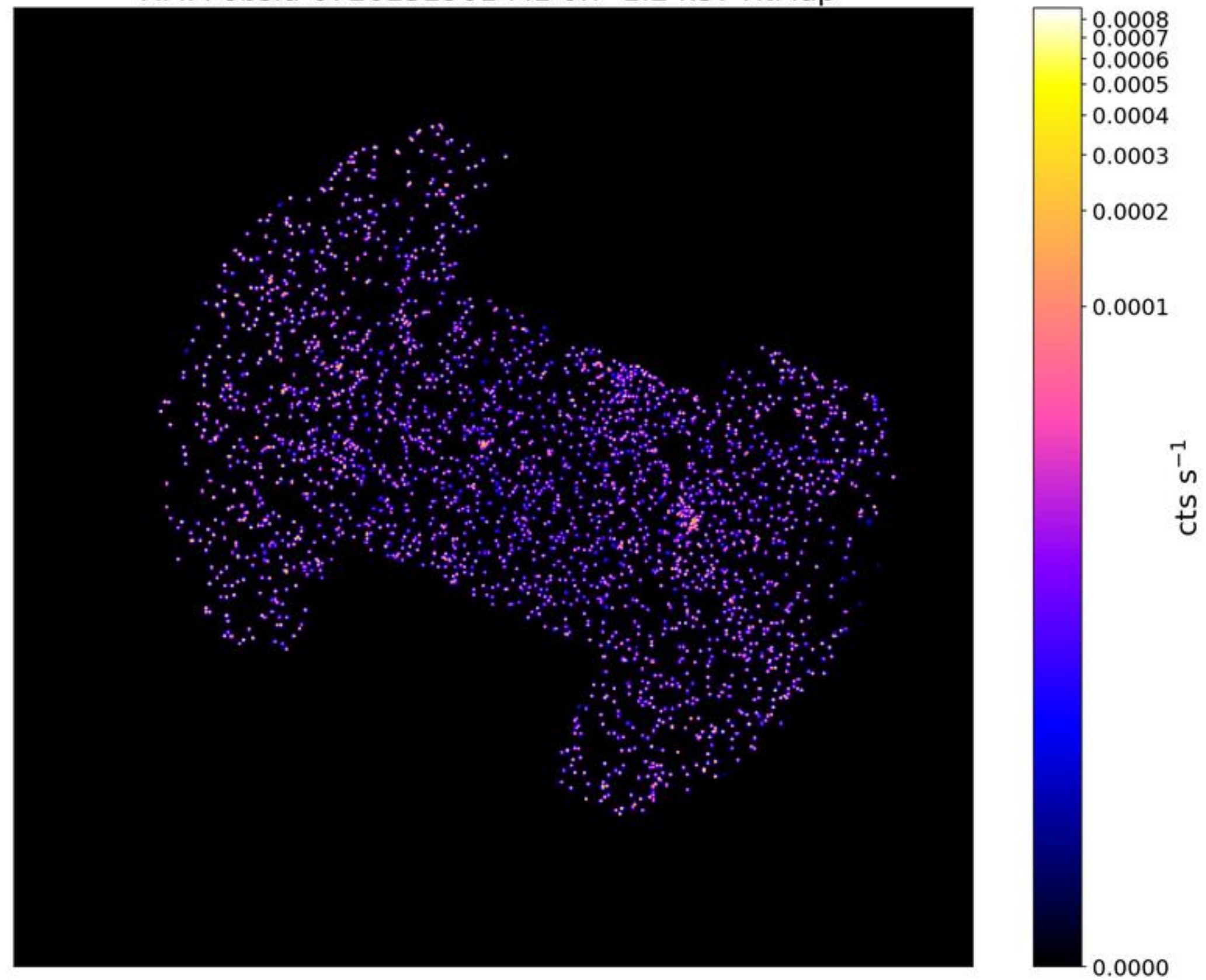
LoVoCCS-103-MCXCI0034.6-0208: \text{Exp}_{\text{clean}}/\text{Exp}_{\text{tot}} = 0.30 XMM obsid-0720252901 M1 0.7-1.2 keV RtMap
