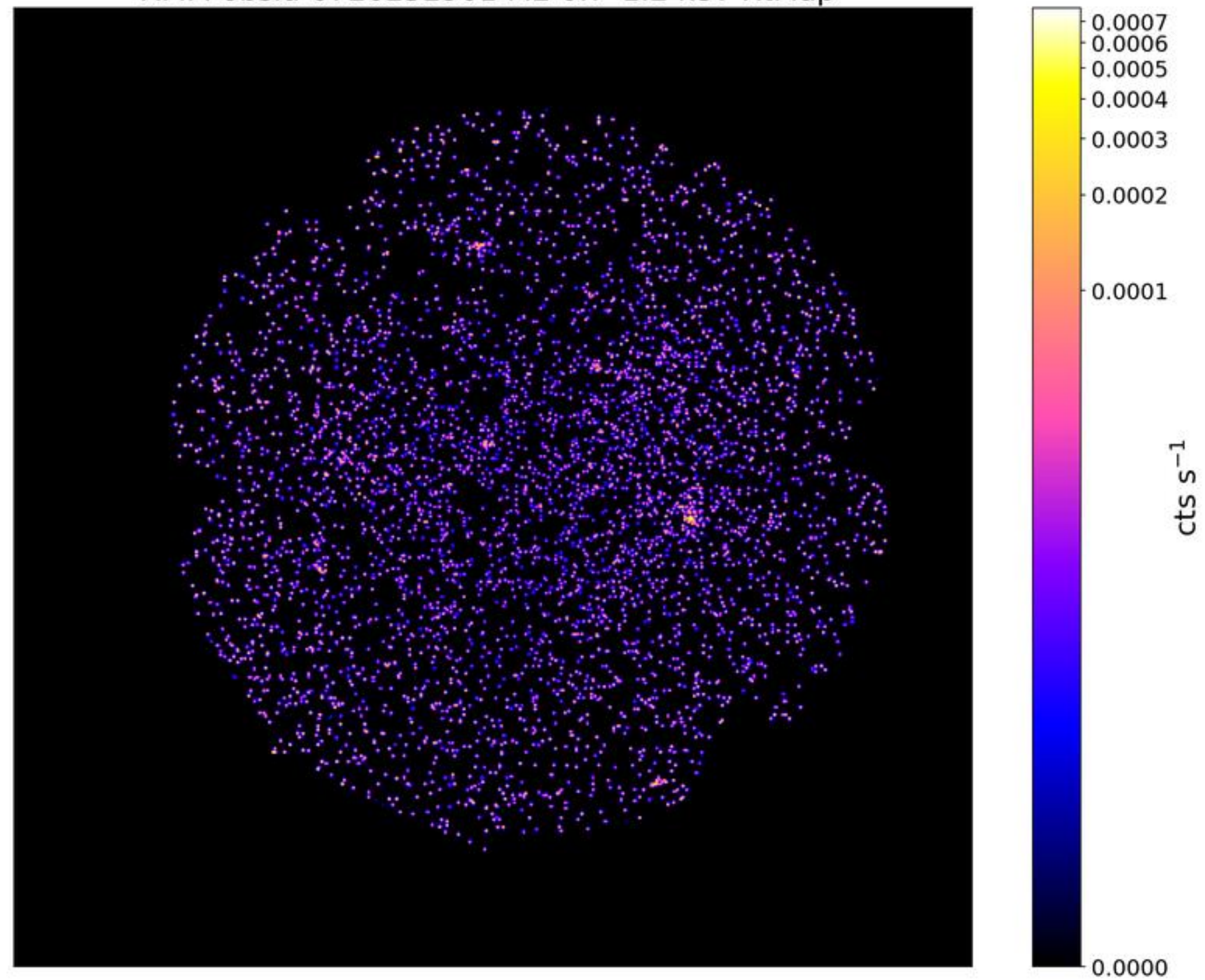
LoVoCCS-103-MCXCI0034.6-0208: \text{Exp}_{\text{clean}}/\text{Exp}_{\text{tot}} = 0.45 XMM obsid-0720252901 M2 0.7-1.2 keV RtMap
