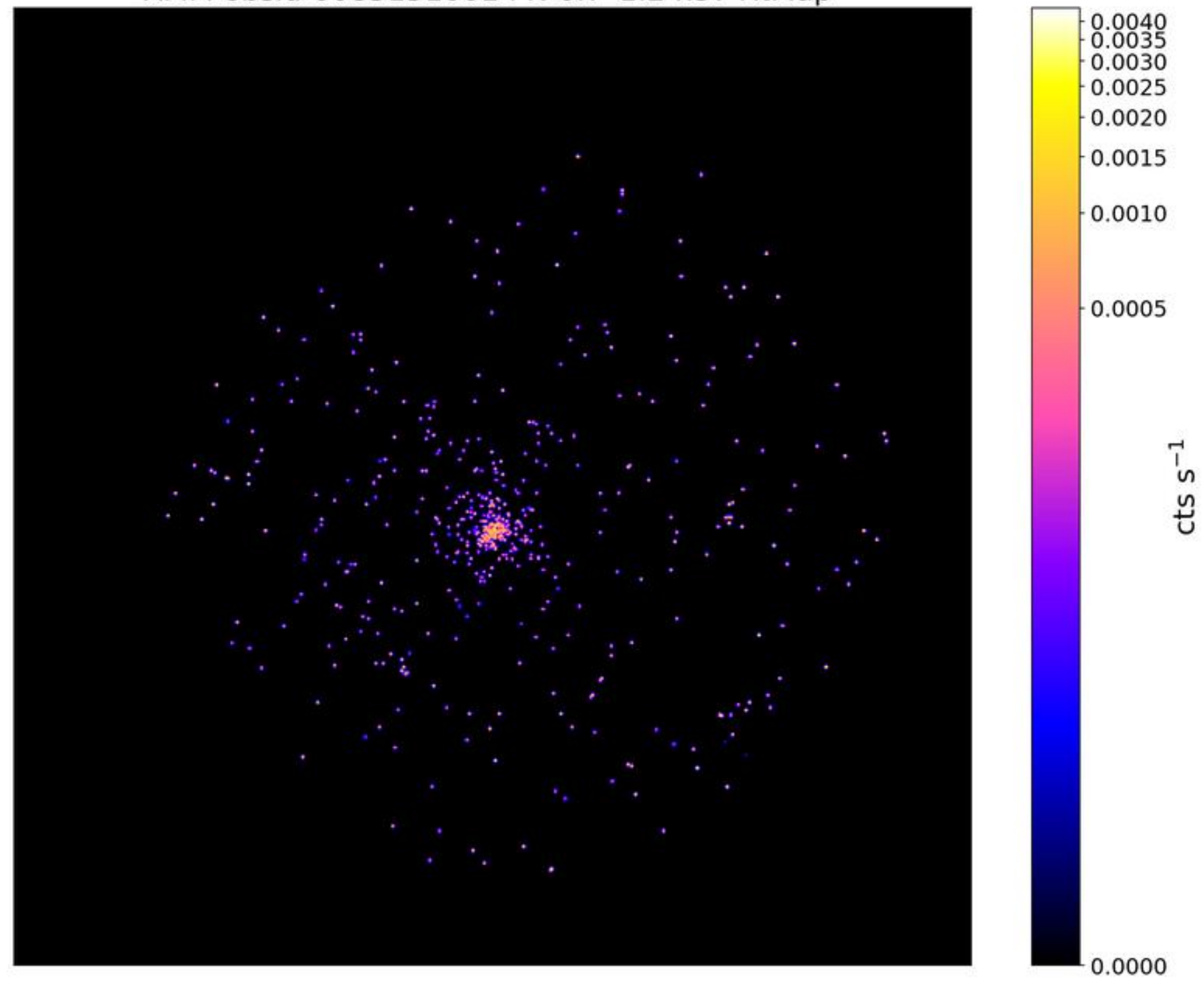
LoVoCCS-118-A2241,B: \text{Exp}_{\text{clean}}/\text{Exp}_{\text{tot}} = 0.04 XMM obsid-0083151001 PN 0.7-1.2 keV RtMap
