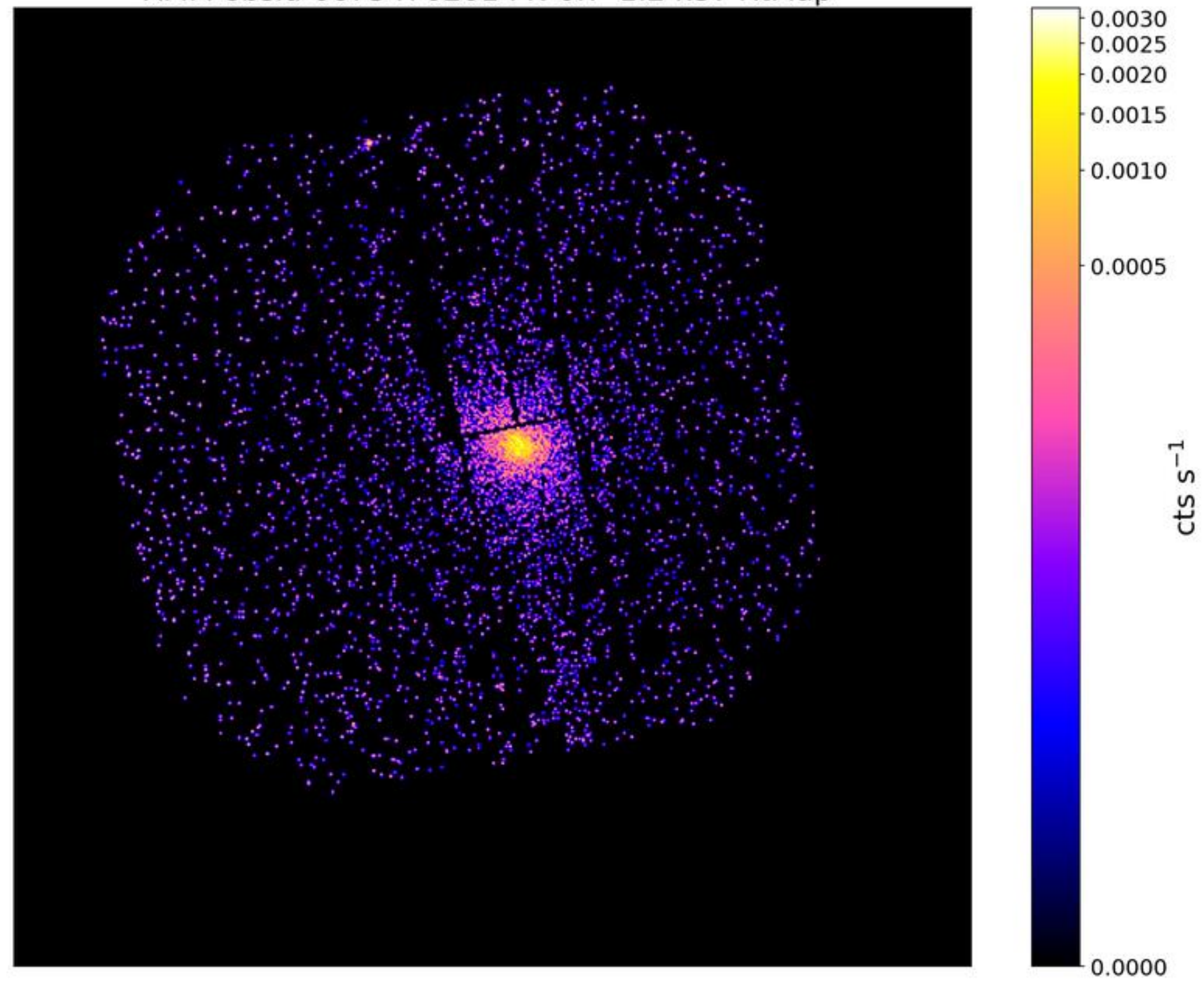
LoVoCCS-20-MCXCI1558.3-1410: \text{Exp}_{\text{clean}}/\text{Exp}_{\text{tot}} = 0.41 XMM obsid-0675470201 PN 0.7-1.2 keV RtMap
