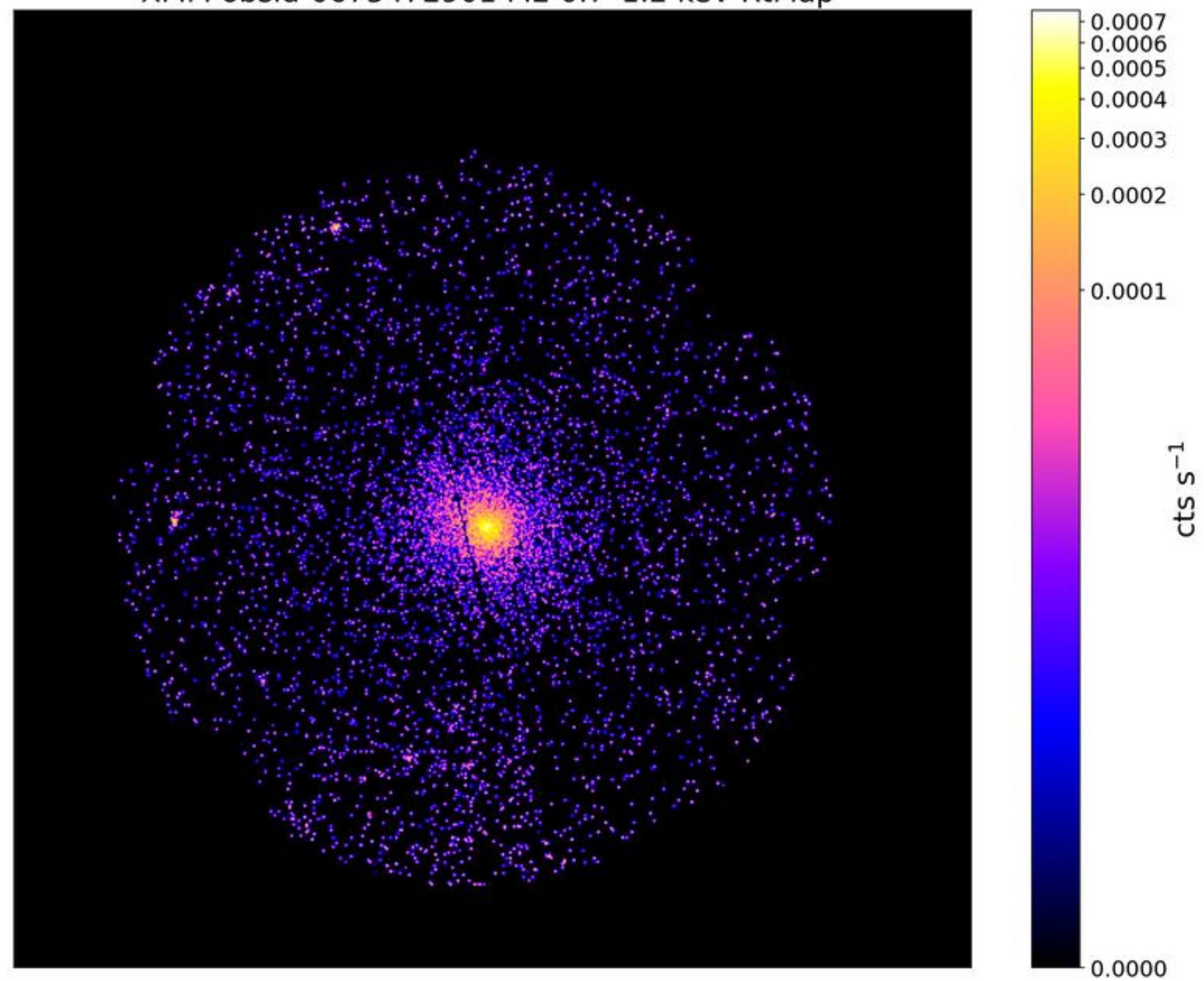
LoVoCCS-20-MCXCI1558.3-1410: \text{Exp}_{\text{clean}}/\text{Exp}_{\text{tot}} = 0.66 XMM obsid-0675472901 M2 0.7-1.2 keV RtMap
