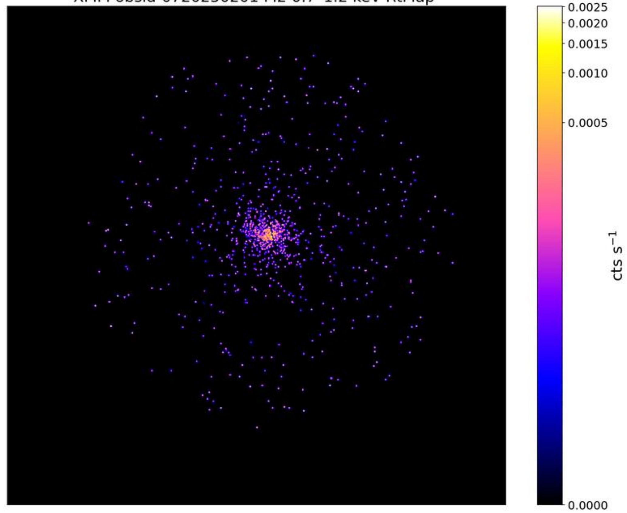
LoVoCCS-20-MCXCI1558.3-1410: \text{Exp}_{\text{clean}}/\text{Exp}_{\text{tot}} = 0.84 XMM obsid-0720250201 M2 0.7-1.2 keV RtMap
