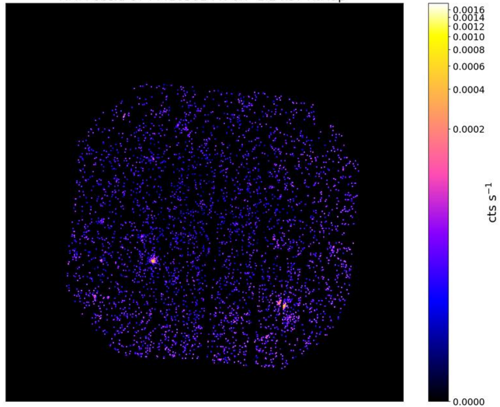
LoVoCCS-23-A2255: \text{Exp}_{\text{clean}}/\text{Exp}_{\text{tot}} = 0.25 XMM obsid-0744410501 PN 0.7-1.2 keV RtMap
