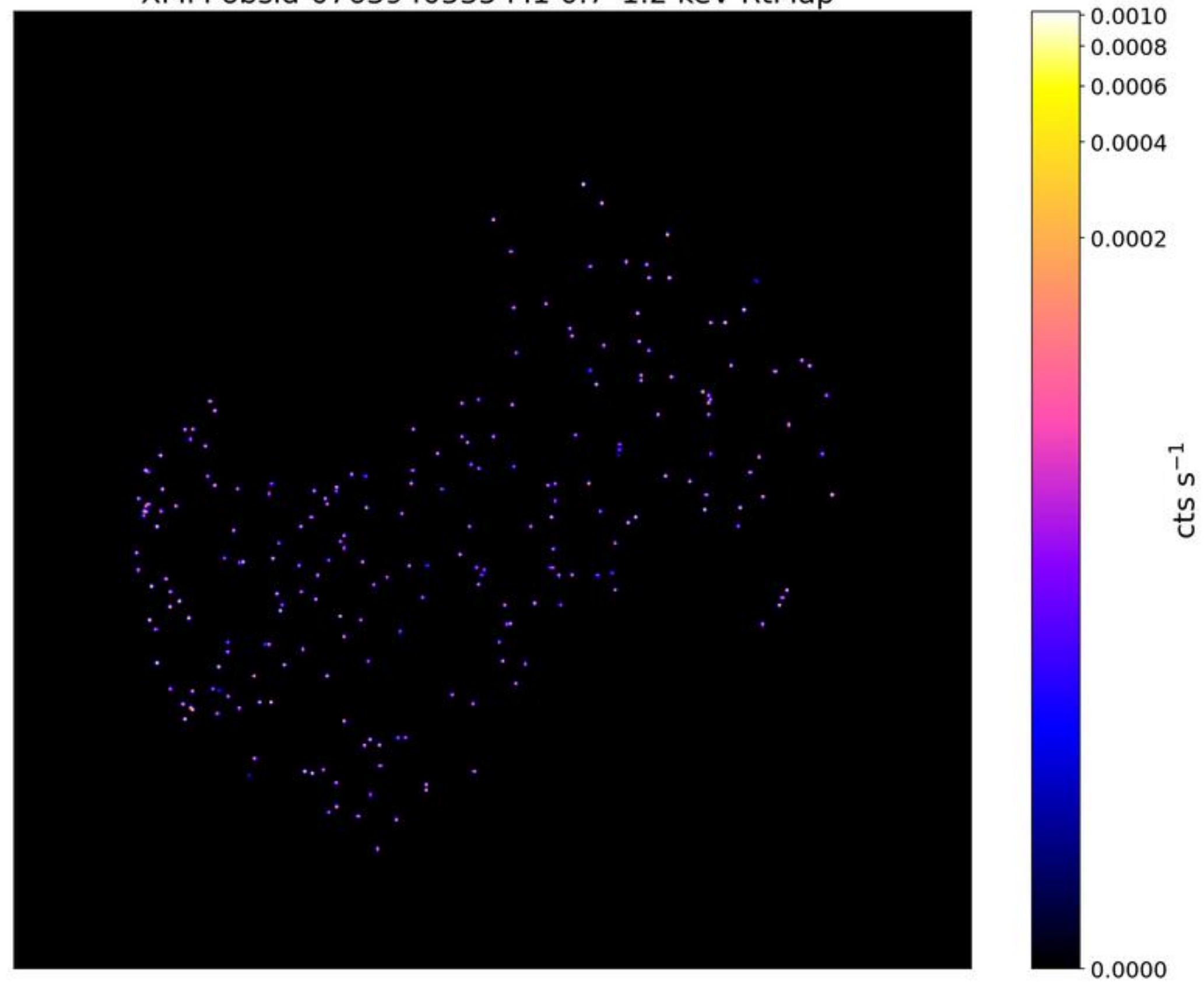
LoVoCCS-40-MCXCI1539.5-8335: \text{Exp}_{\text{clean}}/\text{Exp}_{\text{tot}} = 1.00 XMM obsid-0763940535 M1 0.7-1.2 keV RtMap
