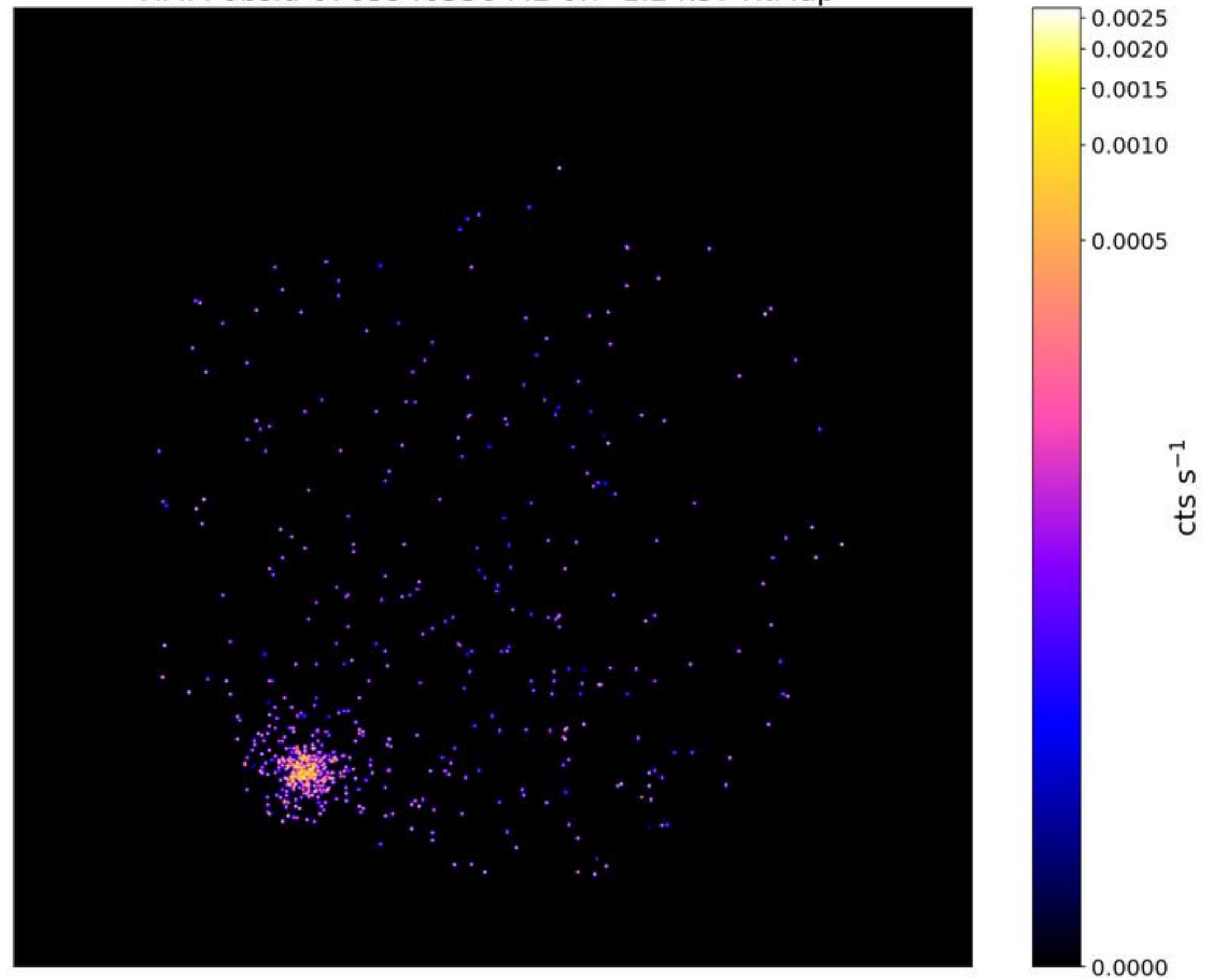
LoVoCCS-40-MCXCI1539.5-8335: \text{Exp}_{\text{clean}}/\text{Exp}_{\text{tot}} = 0.61 XMM obsid-0763940536 M2 0.7-1.2 keV RtMap
