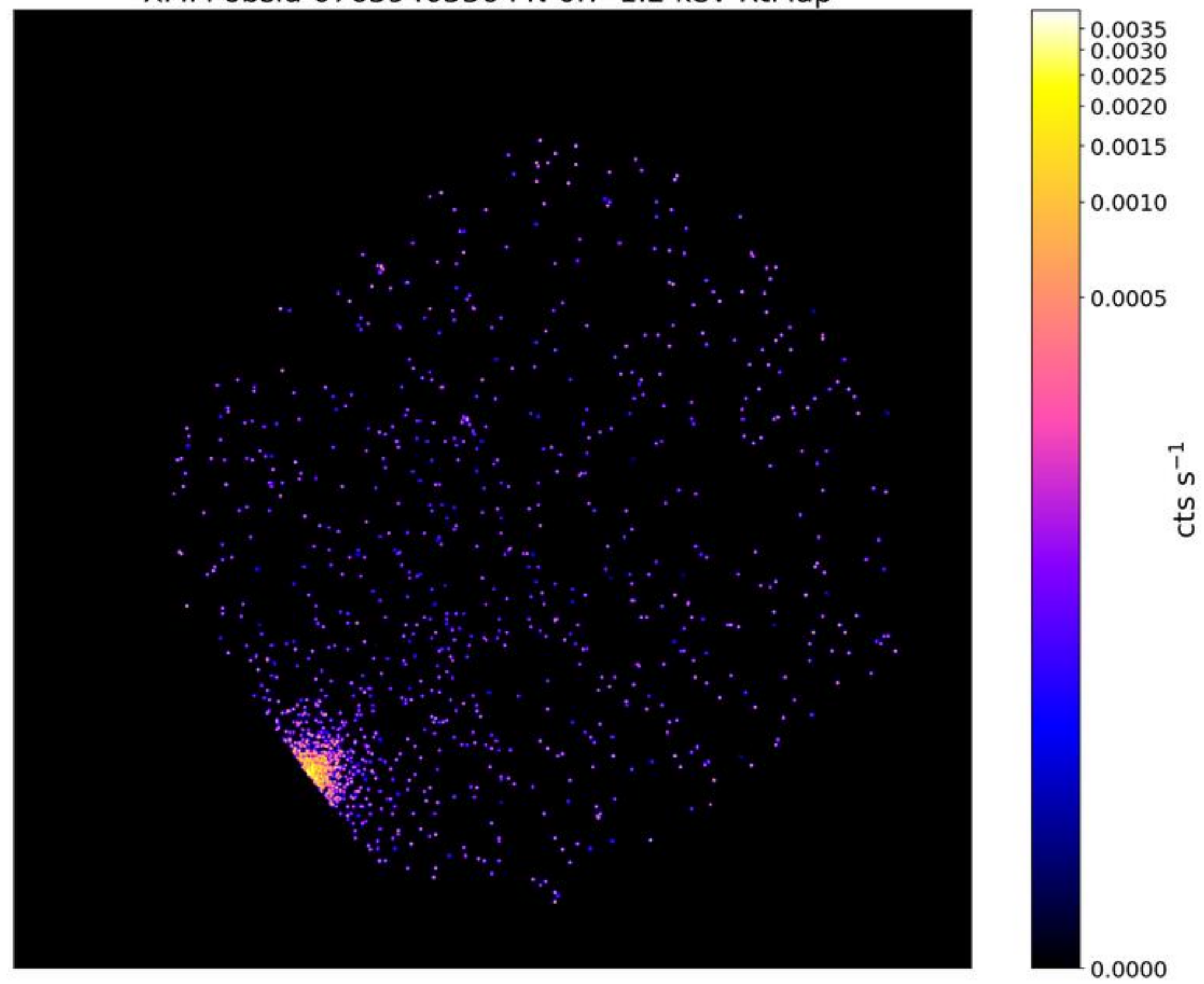
LoVoCCS-40-MCX CJ1539.5-8335: \text{Exp}_{\text{clean}}/\text{Exp}_{\text{tot}} = 0.63 XMM obsid-0763940536 PN 0.7-1.2 keV RtMap
