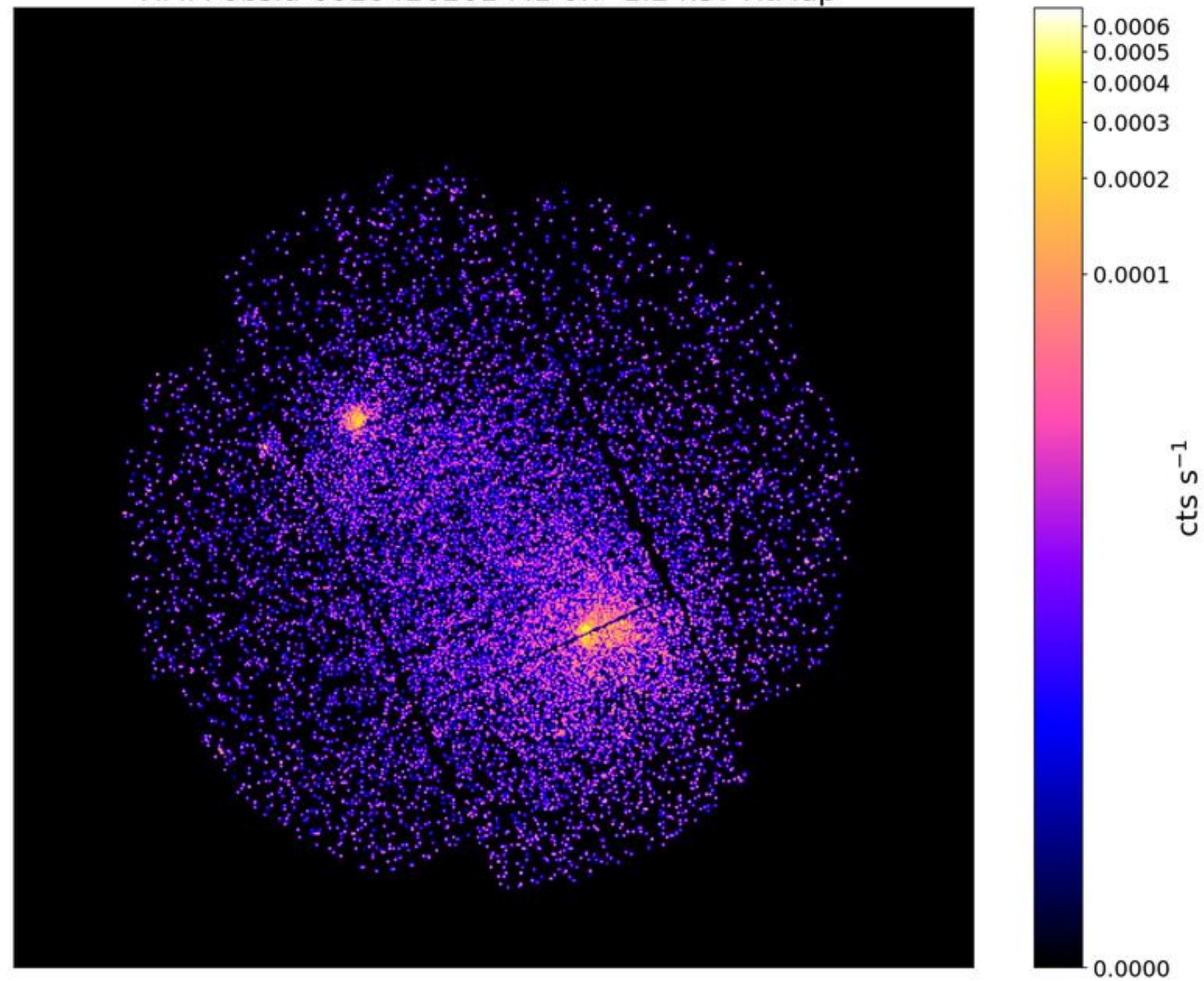
LoVoCCS-48B-A1644: \text{Exp}_{\text{clean}}/\text{Exp}_{\text{tot}} = 0.85 XMM obsid-0010420201 M1 0.7-1.2 keV RtMap
