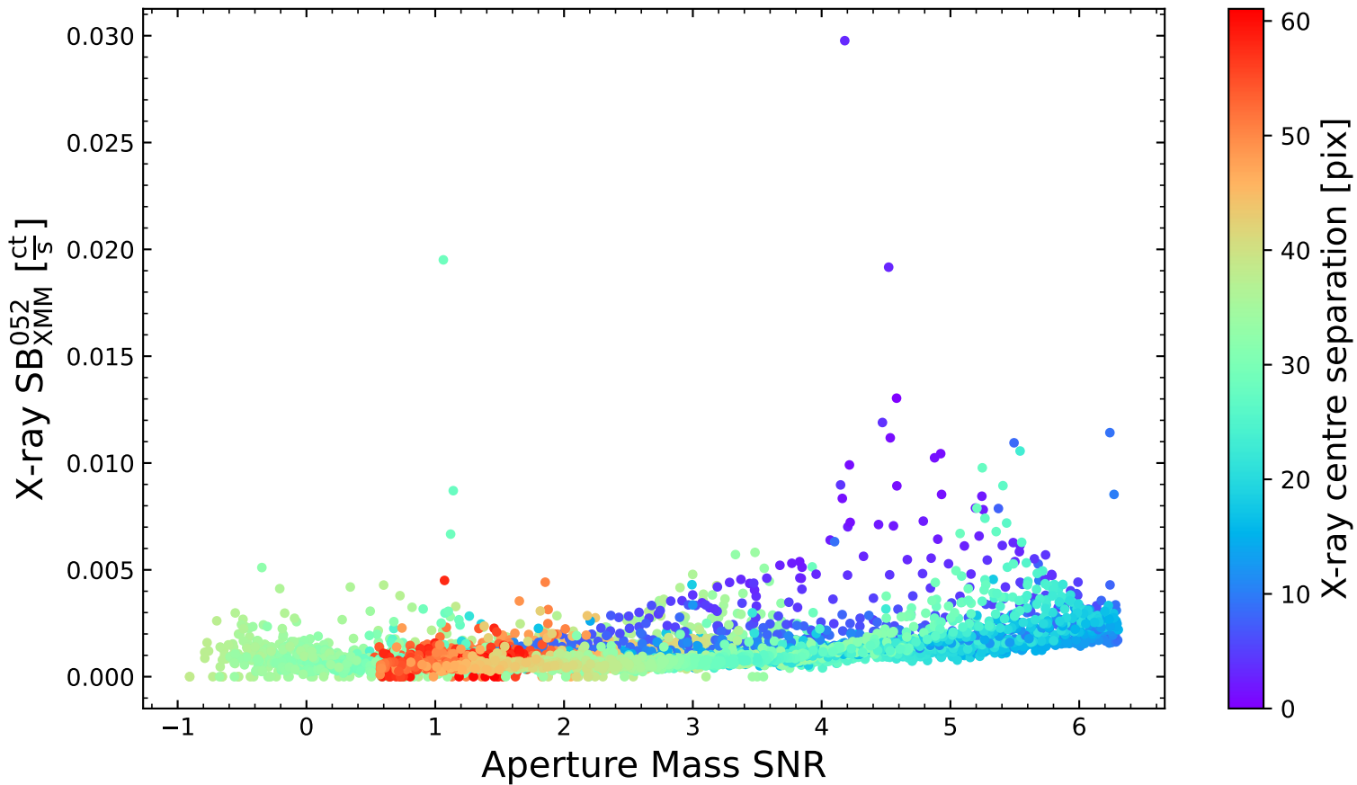
LoVoCCS-121
