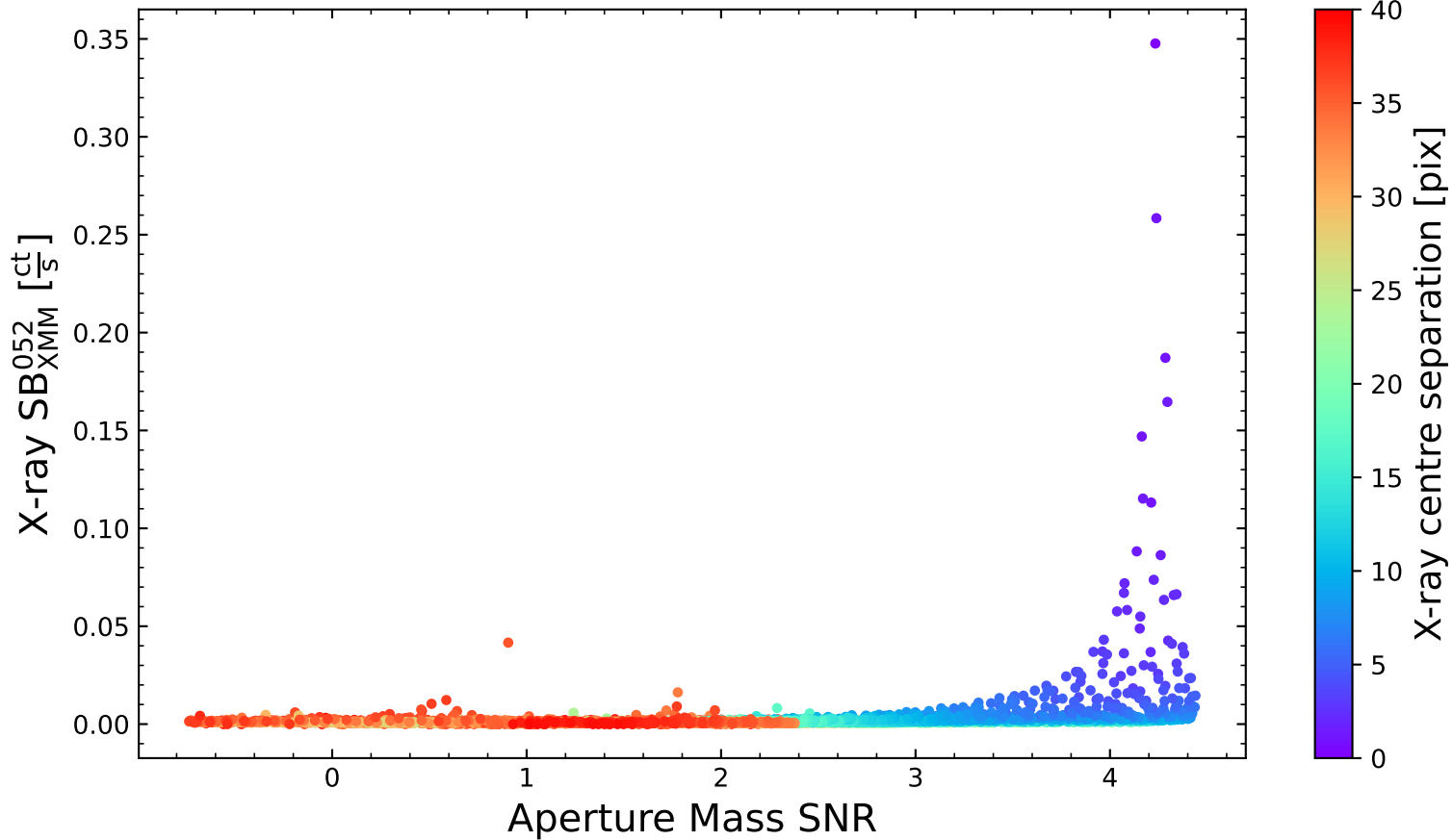
LoVoCCS-13
