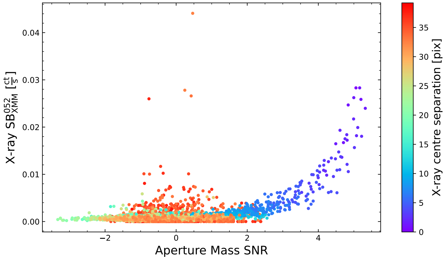
LoVoCCS-80
