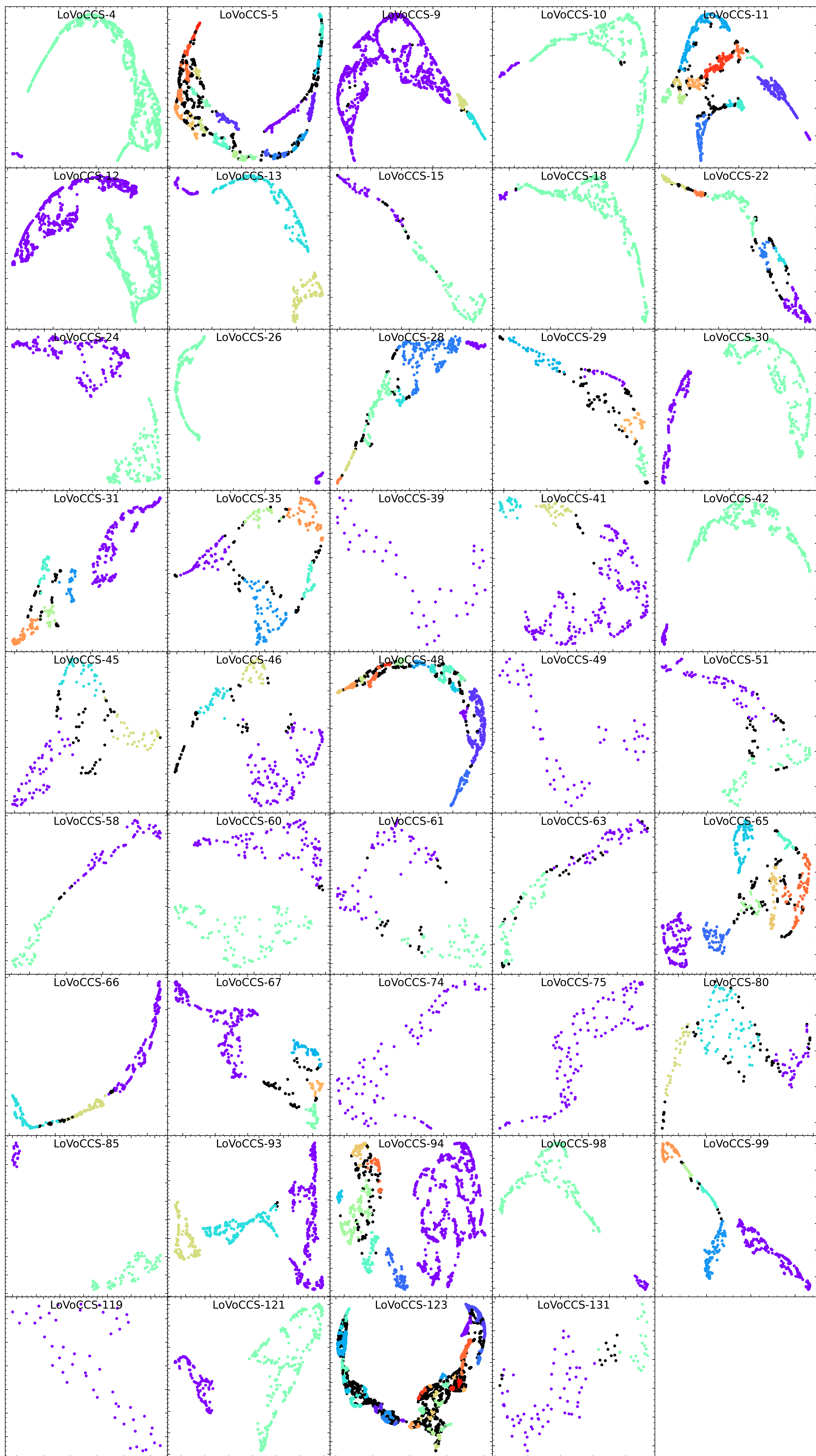
HDBSCAN on UMAP representation of X-ray SB &amp; WL SNR
