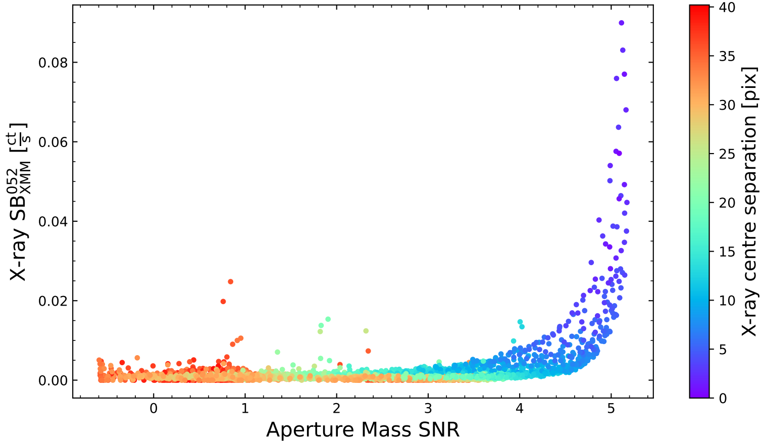
LoVoCCS-10
