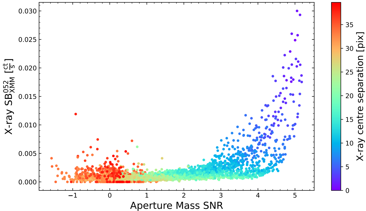
LoVoCCS-31
