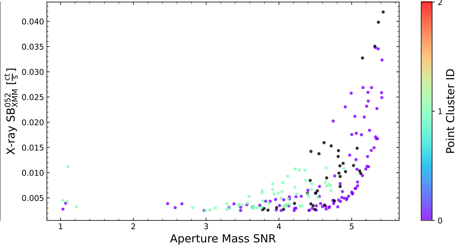
LoVoCCS-29
