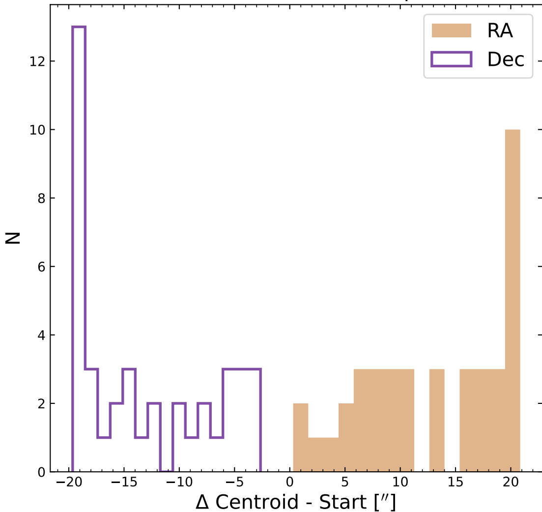
LoVoCCS-35 (100-500 kpc)
