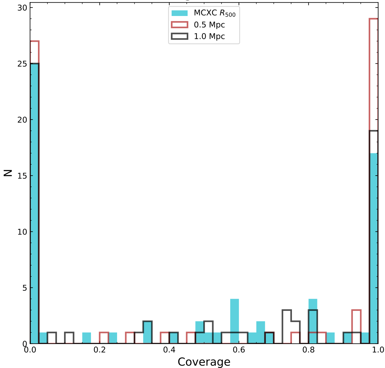
Swift-XRT Coverage Fraction Distribution
