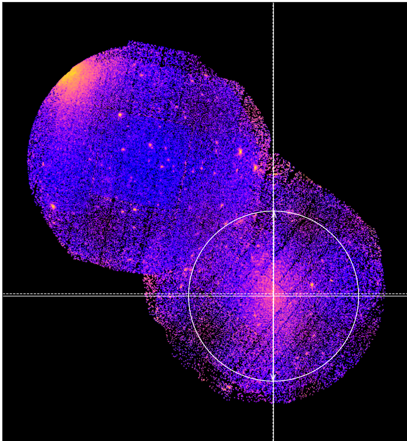
LoVoCCS-134 - Combined 0.5-2.0keV ratemap
