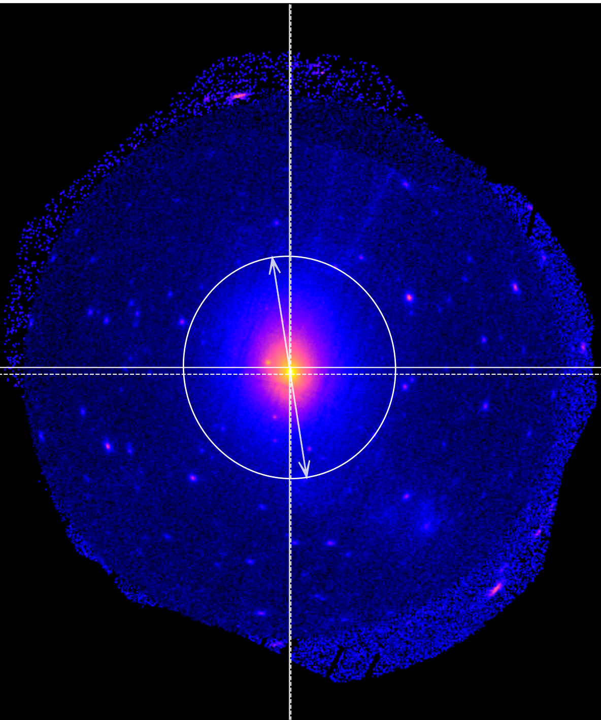
LoVoCCS-13 - Combined 0.5-2.0keV ratemap
