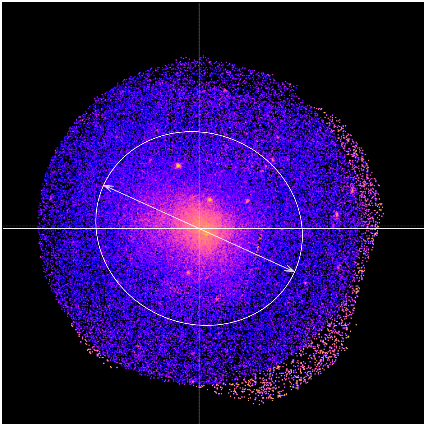
LoVoCCS-42 - Combined 0.5-2.0keV ratemap
