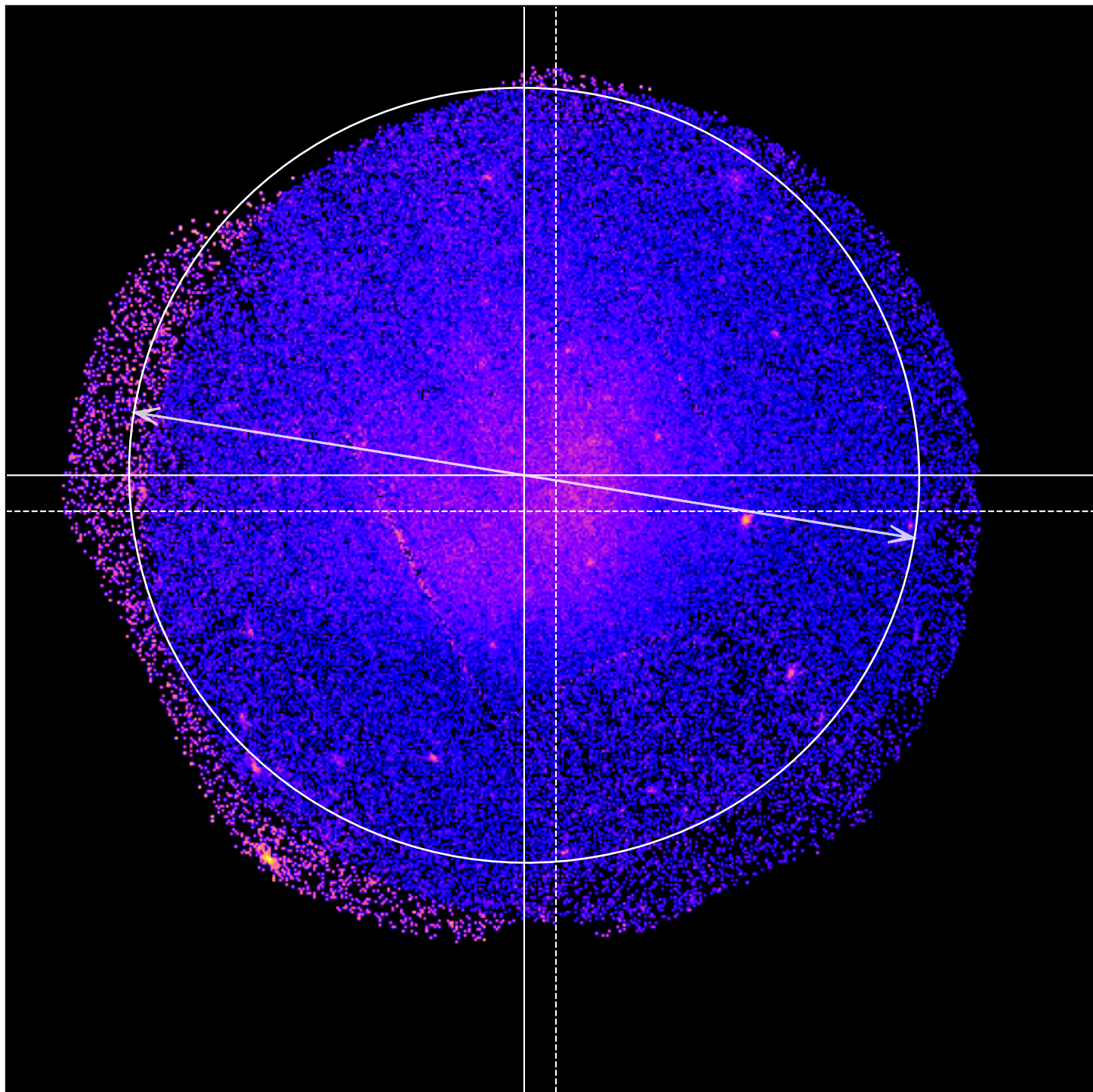
LoVoCCS-65 - Combined 0.5-2.0keV ratemap
