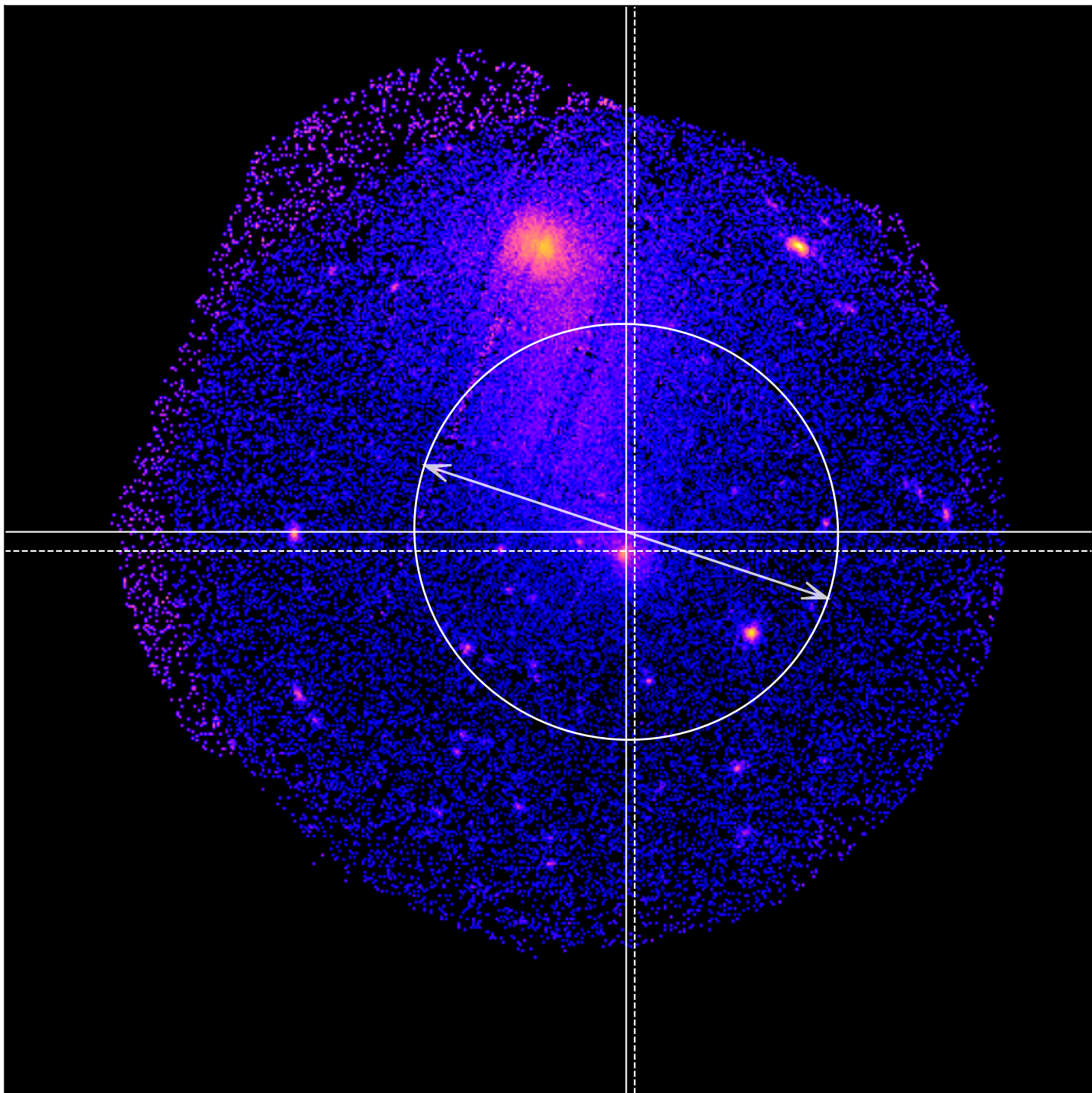
LoVoCCS-66B - Combined 0.5-2.0keV ratemap
