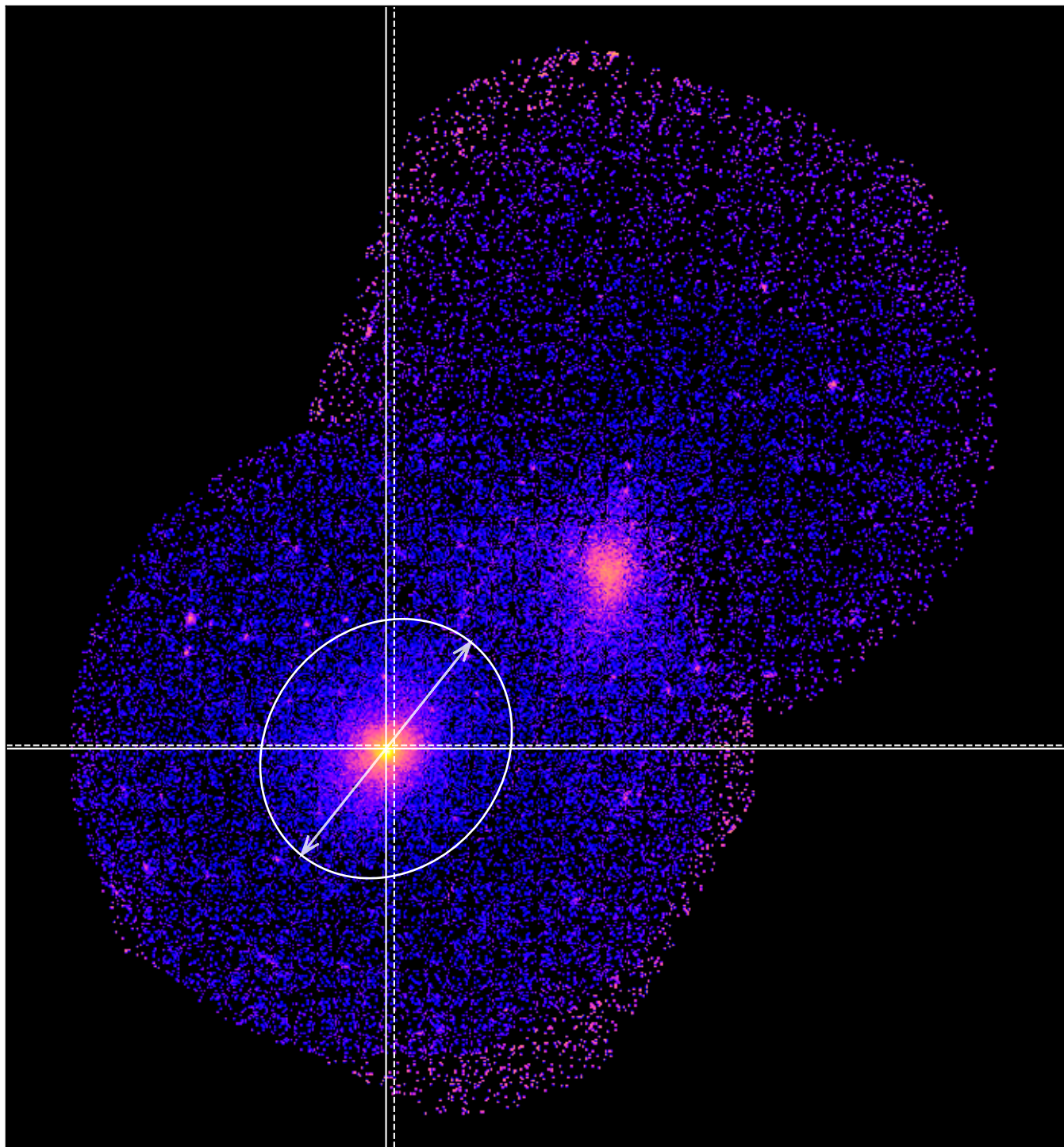
LoVoCCS-76 - Combined 0.5-2.0keV ratemap
