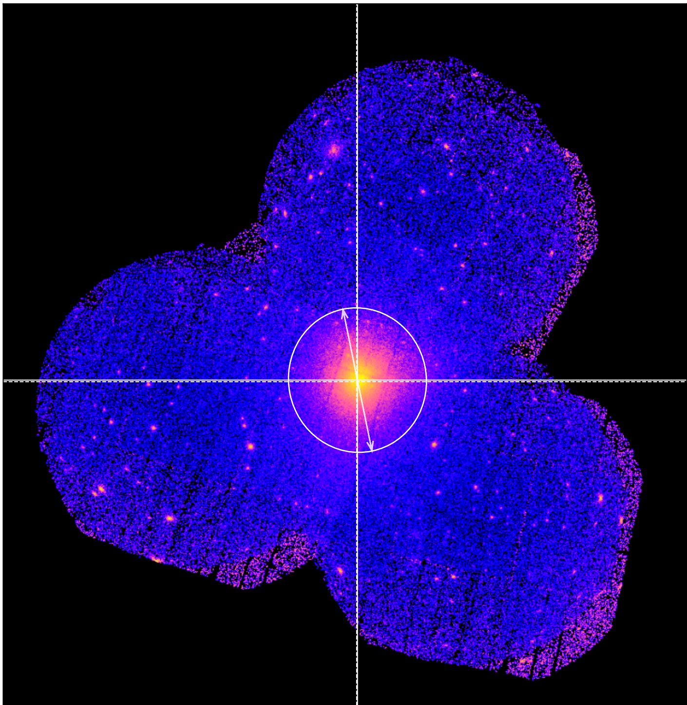
LoVoCCS-7 - Combined 0.5-2.0keV ratemap
