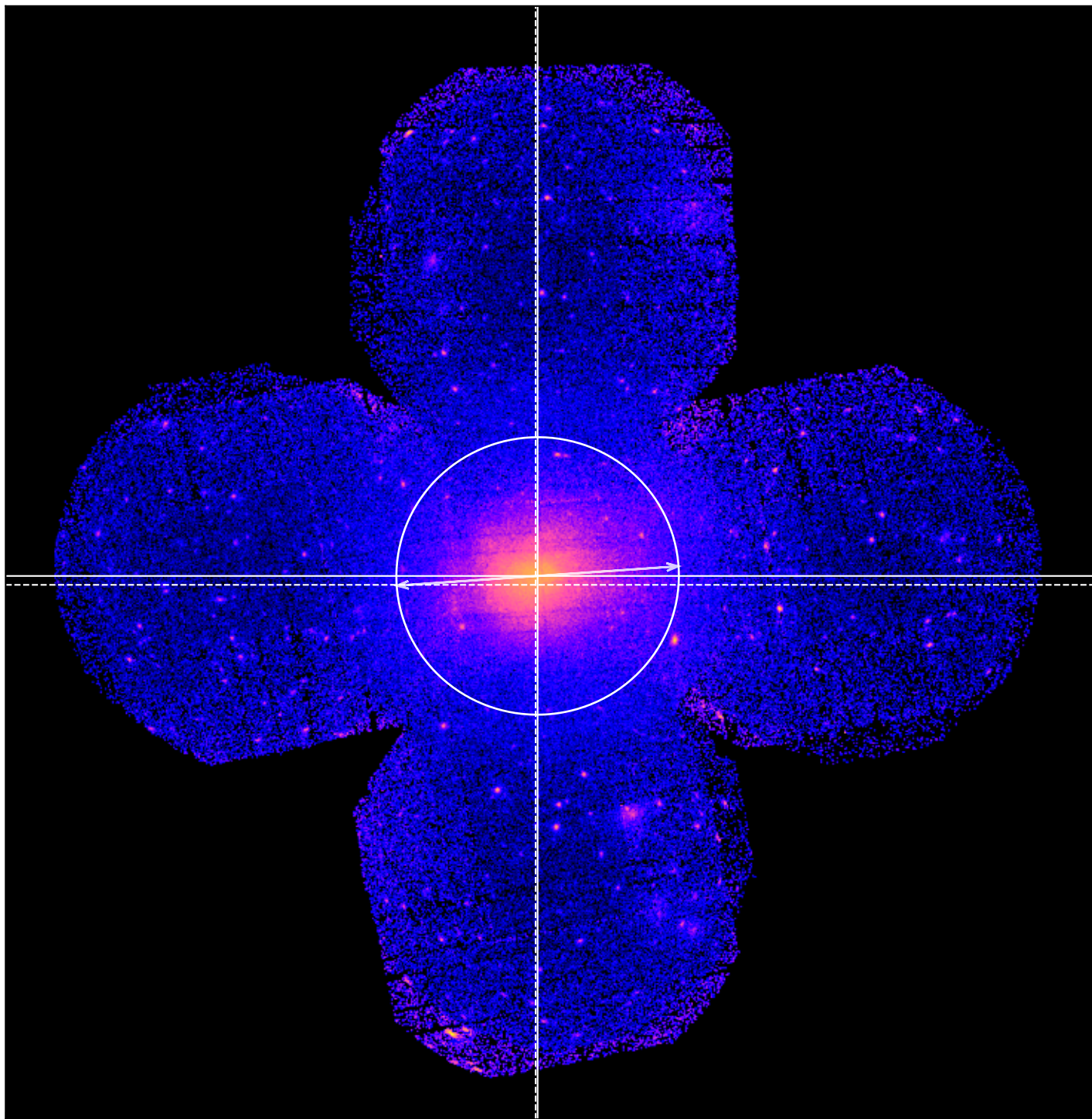
LoVoCCS-27 - Combined 0.5-2.0keV ratemap
