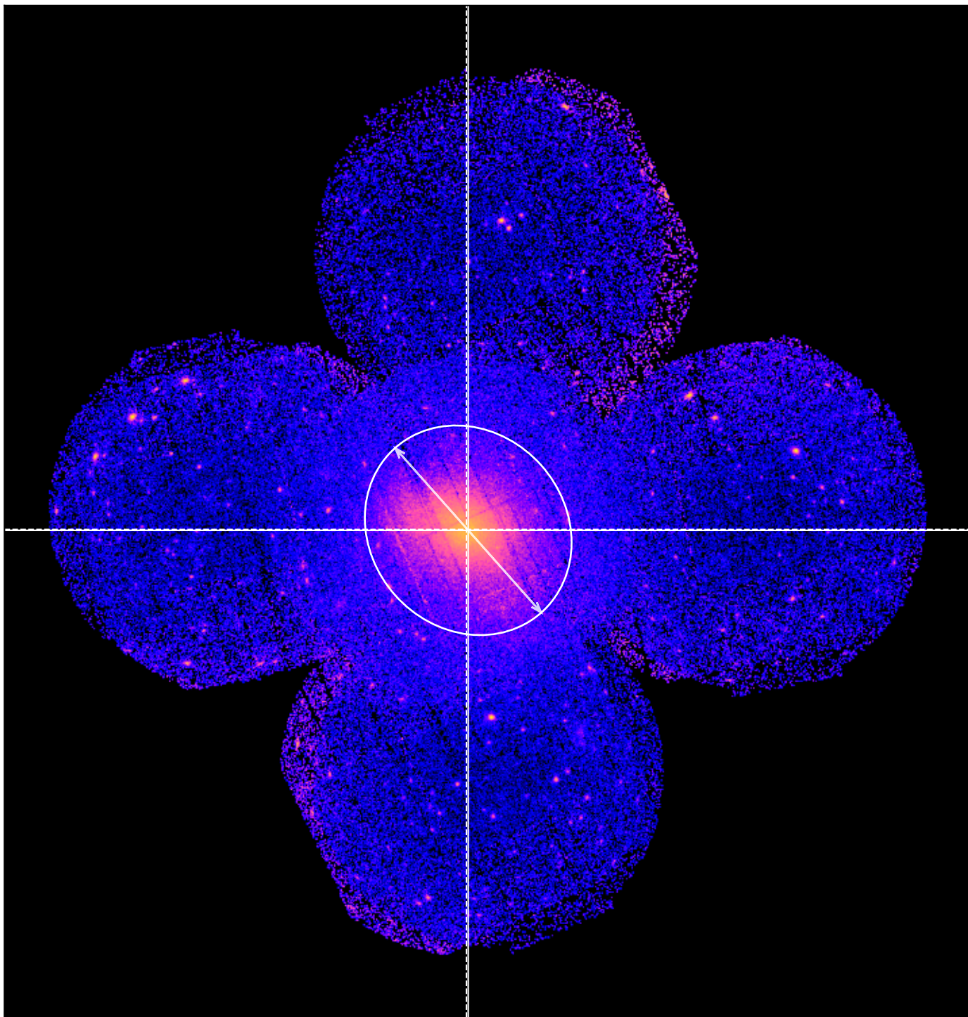
LoVoCCS-28 - Combined 0.5-2.0keV ratemap
