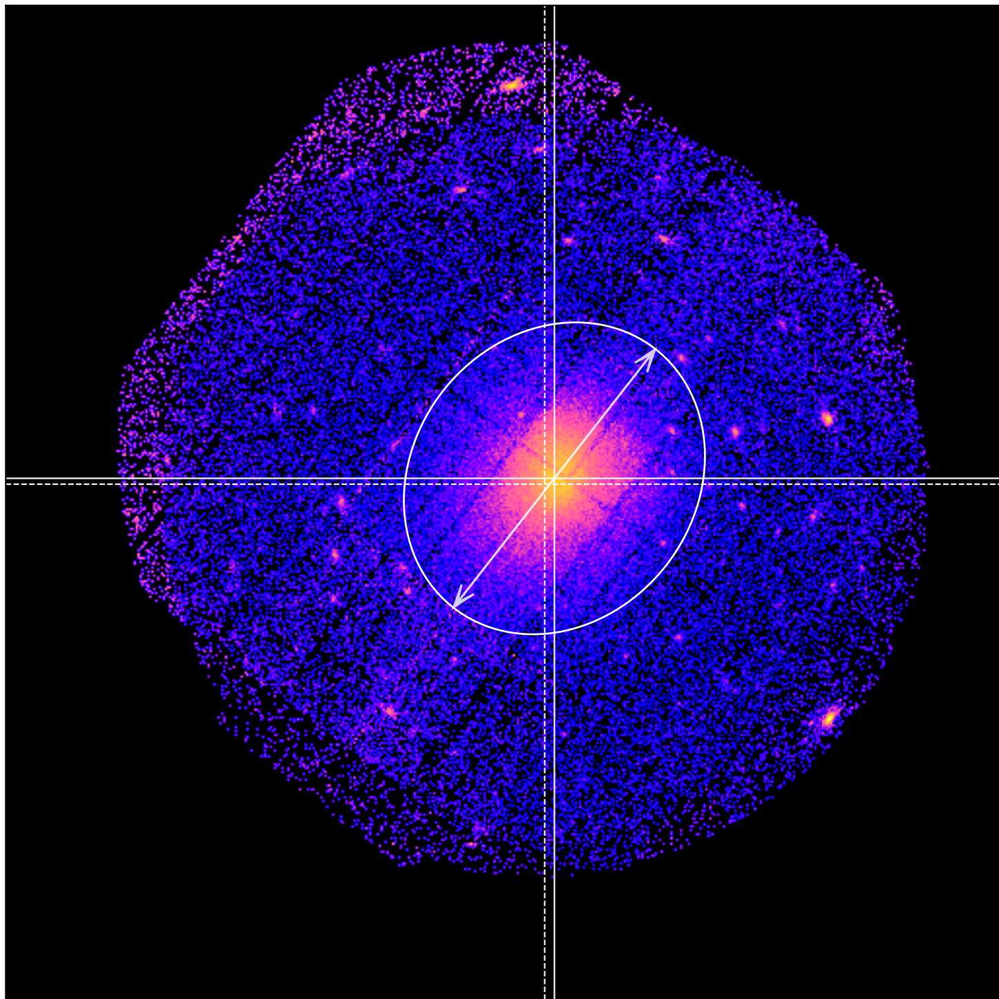
LoVoCCS-29 - Combined 0.5-2.0keV ratemap
