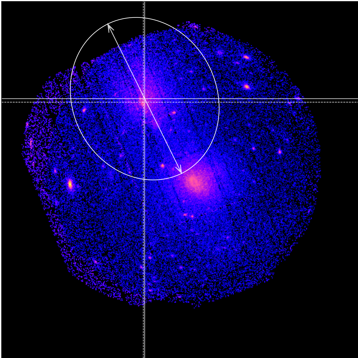
LoVoCCS-41B - Combined 0.5-2.0keV ratemap
