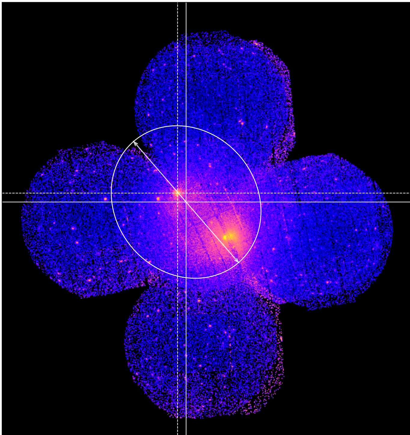
LoVoCCS-48B - Combined 0.5-2.0keV ratemap
