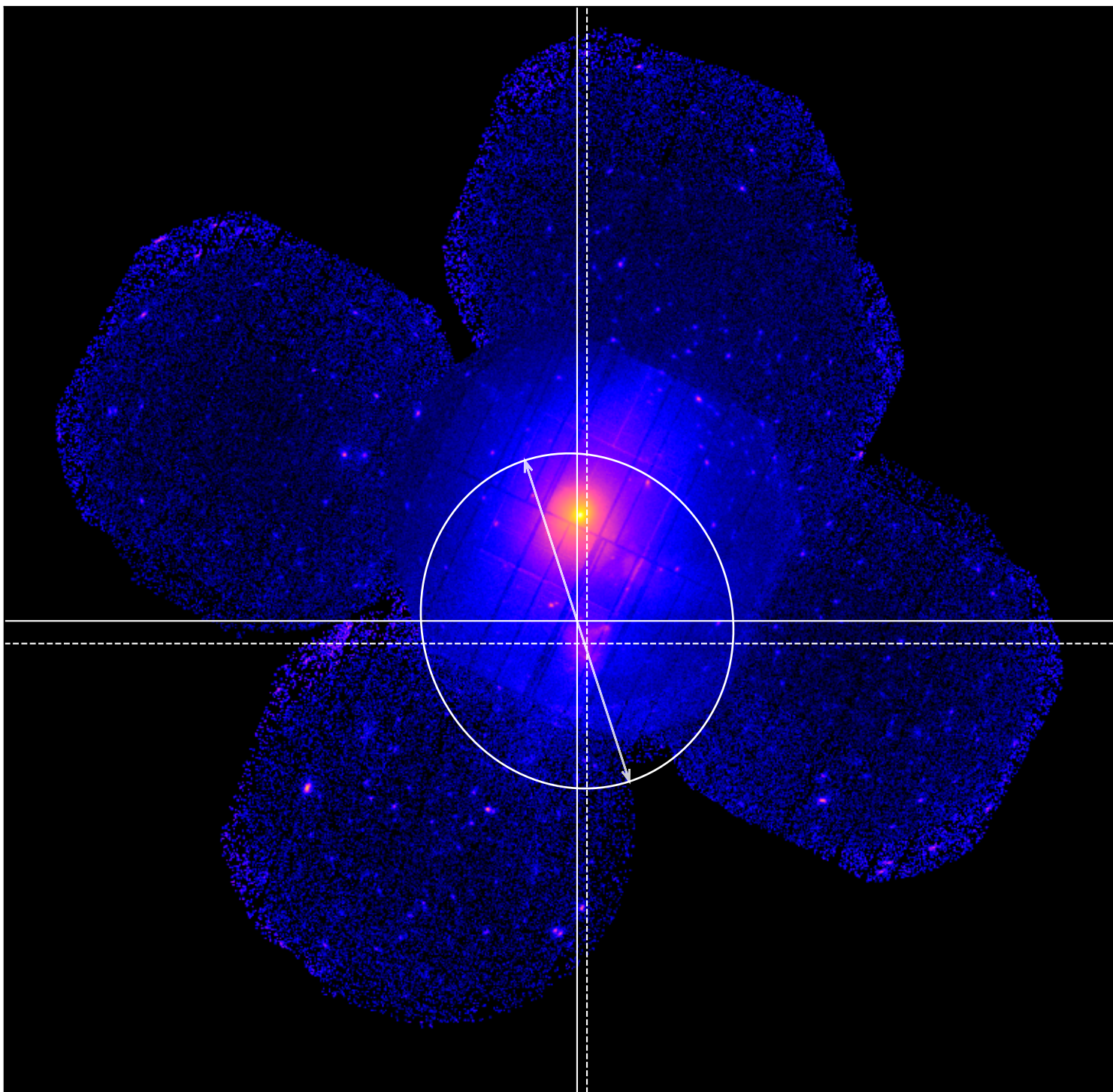
LoVoCCS-4B - Combined 0.5-2.0keV ratemap
