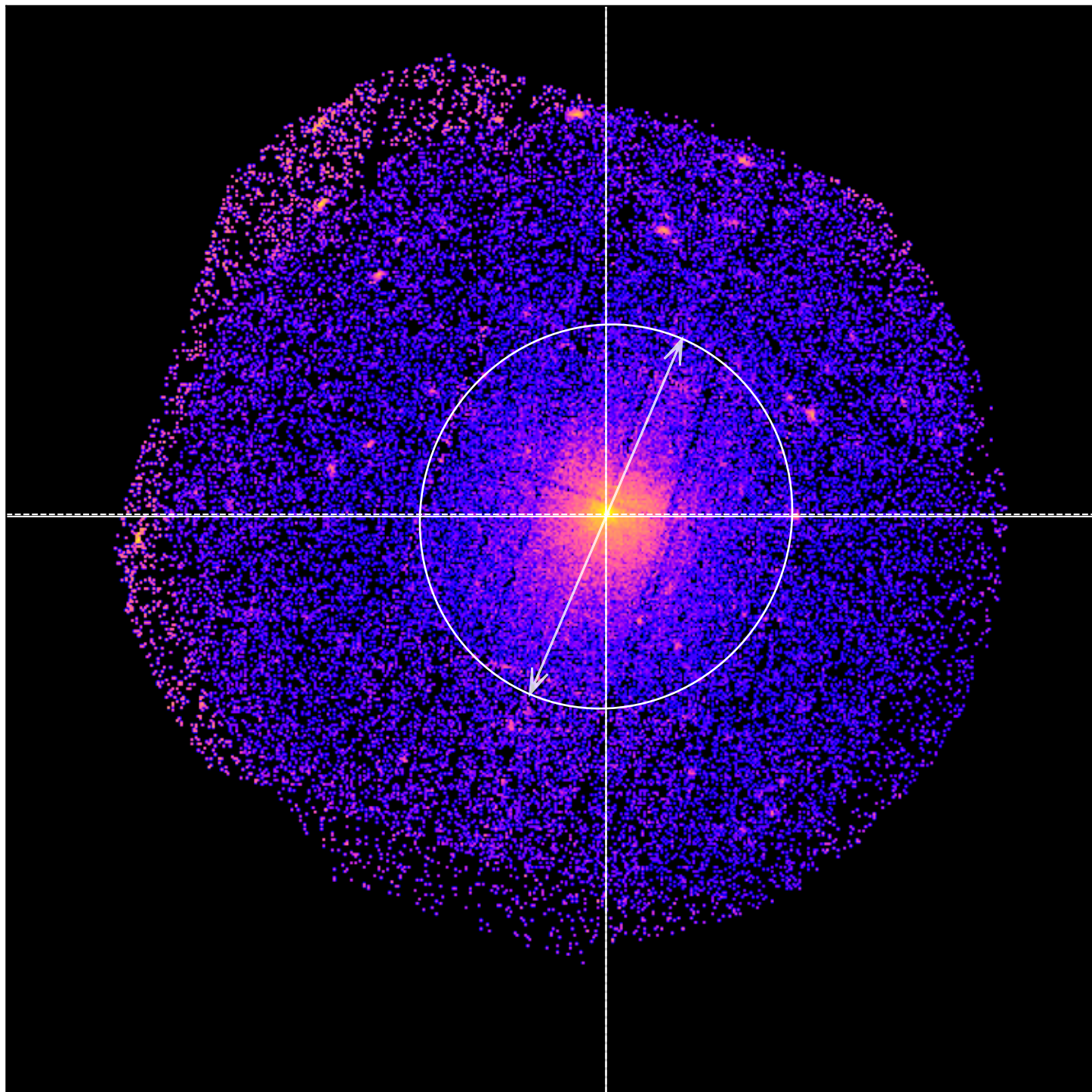
LoVoCCS-51 - Combined 0.5-2.0keV ratemap
