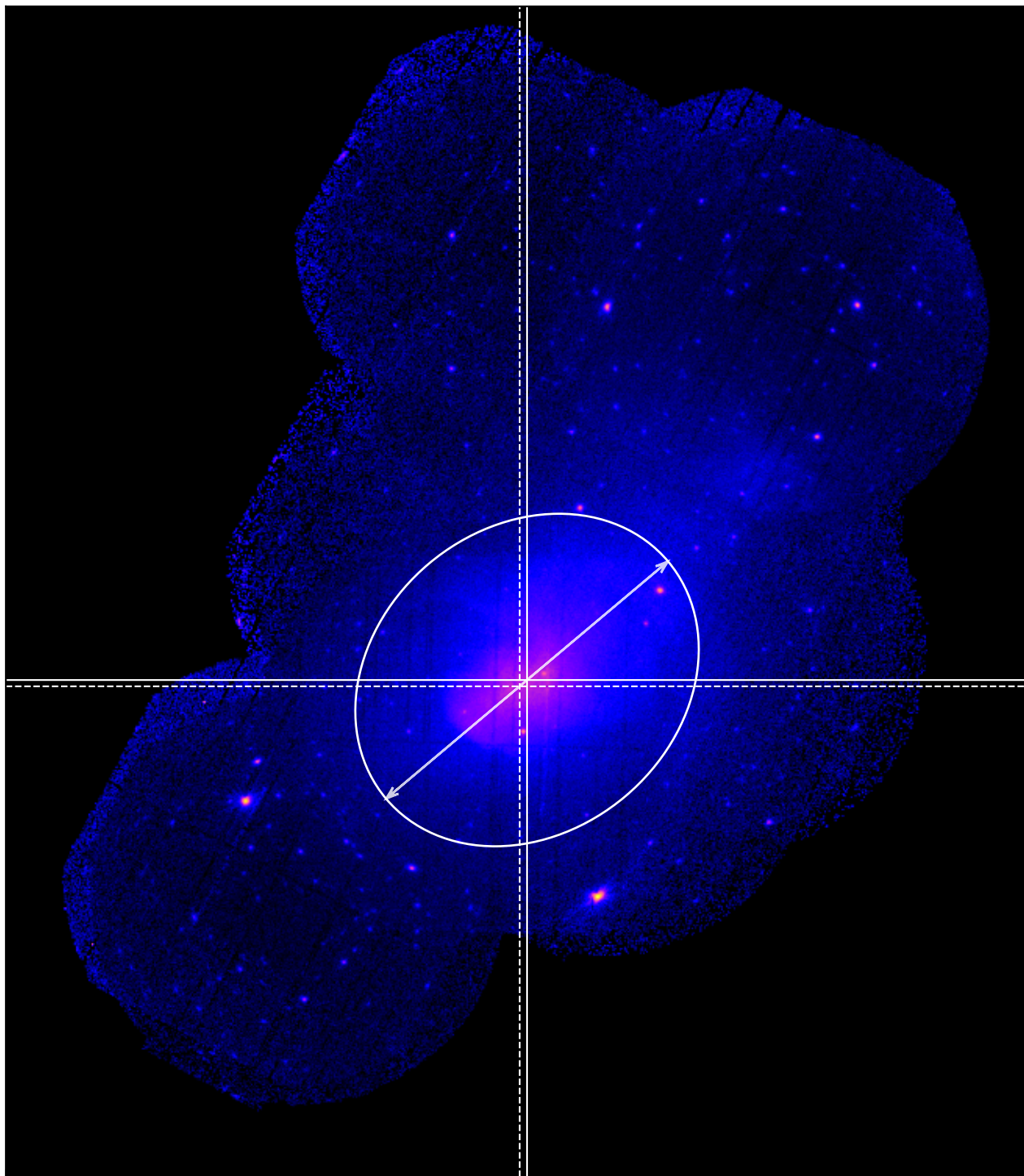
LoVoCCS-5 - Combined 0.5-2.0keV ratemap
