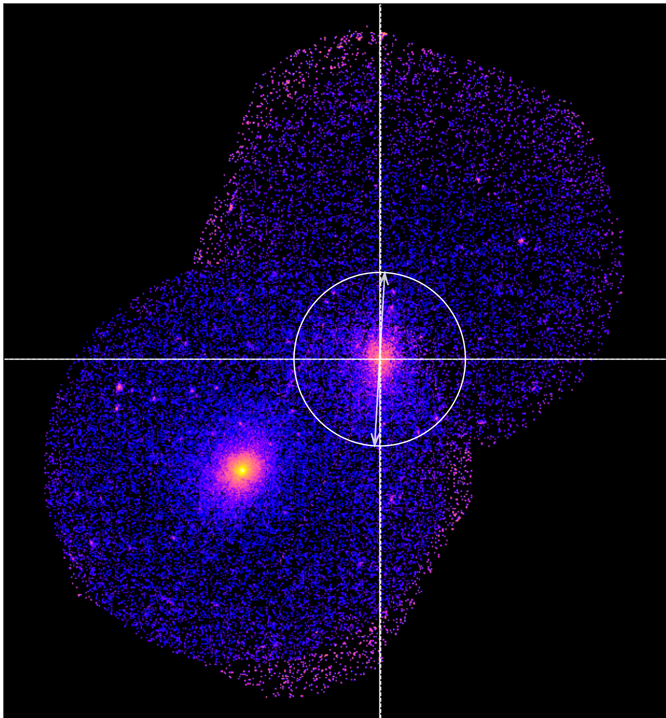
LoVoCCS-89 - Combined 0.5-2.0keV ratemap
