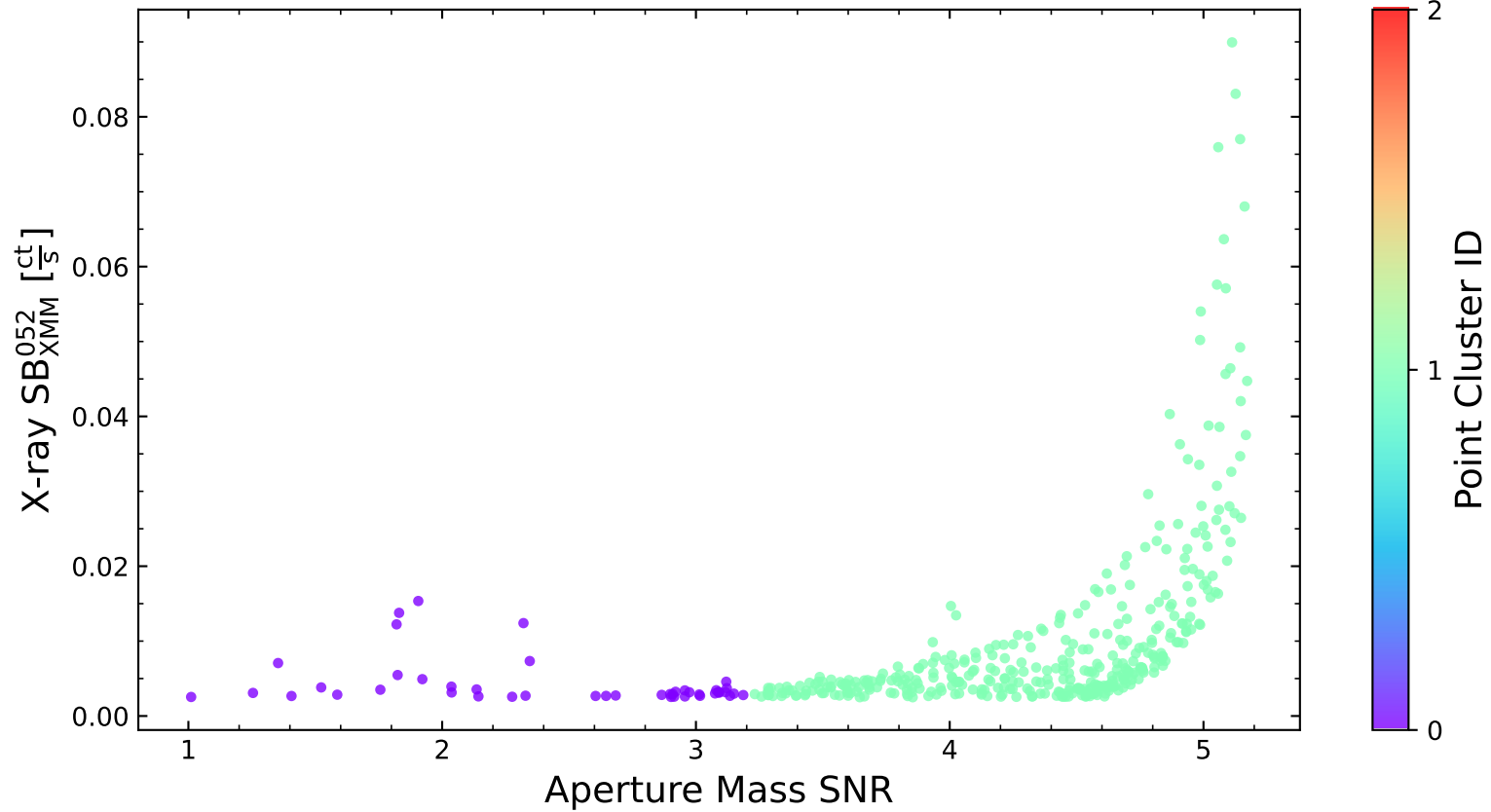
LoVoCCS-10
