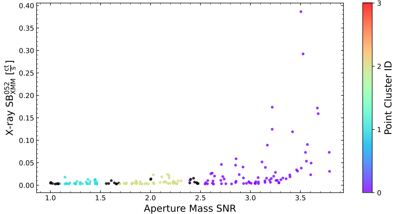
LoVoCCS-15
