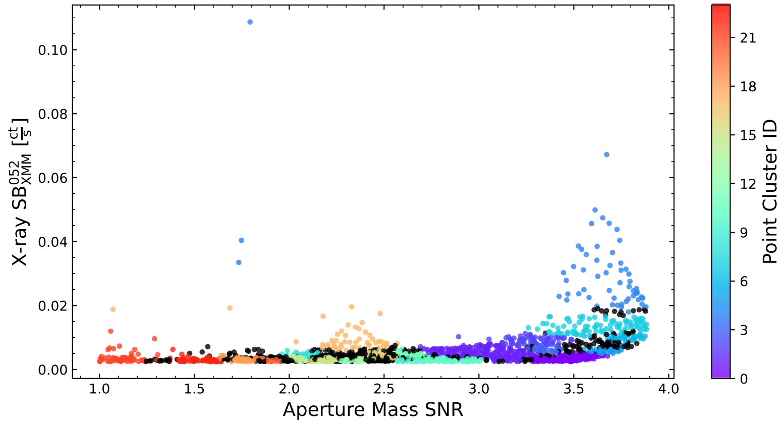
LoVoCCS-21
