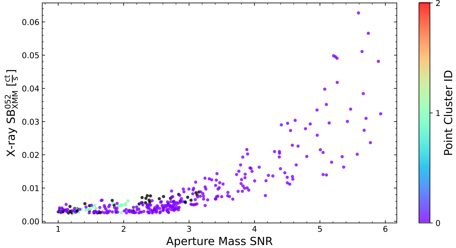
LoVoCCS-7
