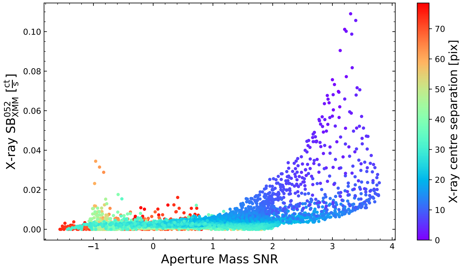
LoVoCCS-12
