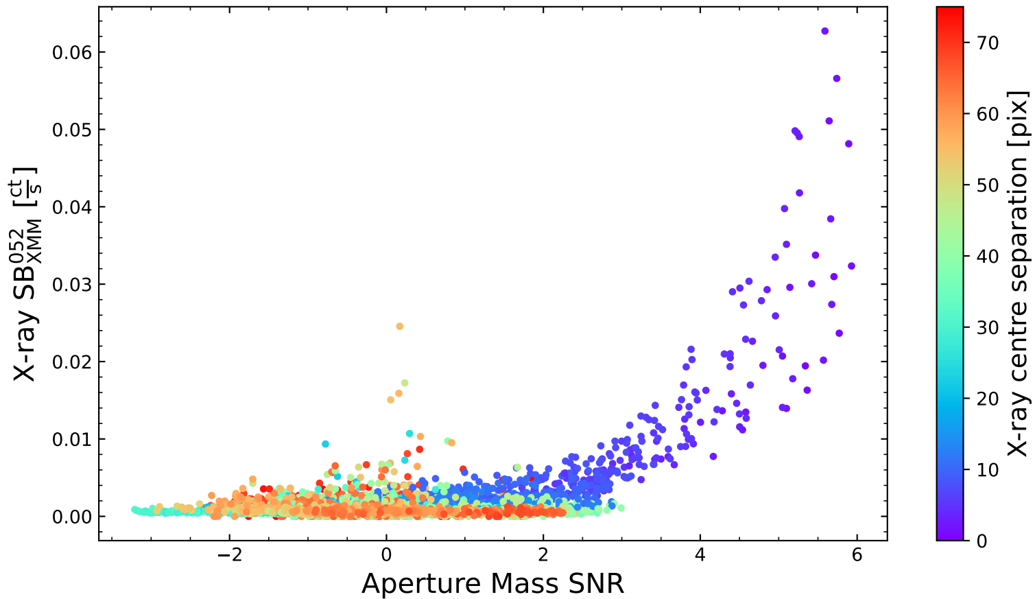
LoVoCCS-7
