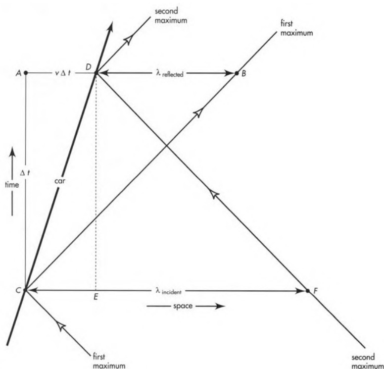
Figure 5.E.5: Worldlines of approaching car and two radar wave maxima that reflect from the car. The speed of the car is greatly exaggerated.
