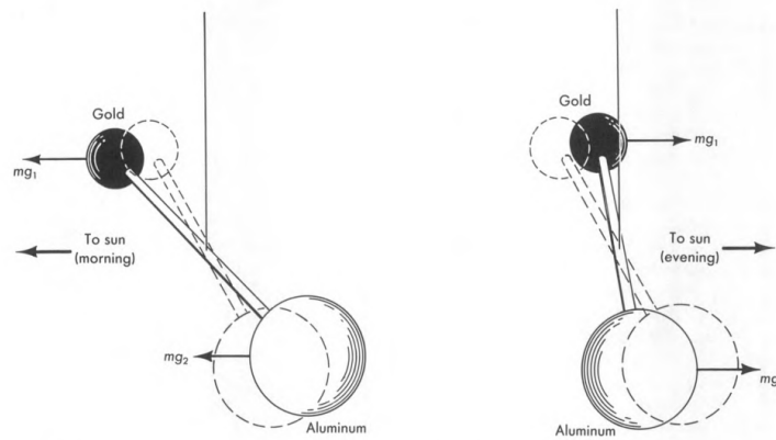
Figure 2.E.4: second figure . Schematic diagram of the Dicke experiment. Left : Hypothetical effect: morning. Right : Hypothetical effect: evening. Any difference in the gravitational acceleration of Sun for gold and aluminum should result in opposite sense of net torque on torsion pendulum in the evening compared with the morning. The large aluminum ball has the same mass as the small high-density gold ball.
