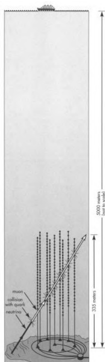
Figure 3.E.4: Use of Čerenkov radiation for indirect detection of neutrinos in the Deep Underwater Muon and Neutrino Detector (DUMAND) 30 kilometers off Keahole Point on the island of Hawaii. Neutrinos have no electric charge and their mass, if any, has so far escaped detection (Box 8-1). Neutrinos interact extremely weakly with matter, passing through Earth with almost no collisions. Indeed, the DUMAND detector array selects for analysis only neutrinos that come upward through Earth. In this way Earth itself acts as a shield to eliminate all other cosmic-ray particles.
