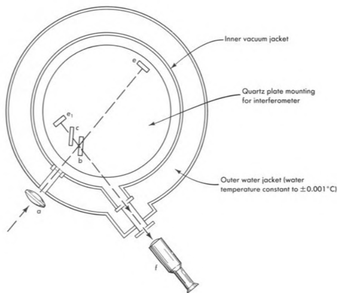
Figure 3.E.8: Schematic diagram of apparatus used for the Kennedy- Thorndike experiment. Parts of the interferometer have been labeled with letters corresponding to those used in describing the Michelson-Morley interferometer (Exercise 3-12). The experimenters went to great lengths to insure the optical and mechanical stability of their apparatus. The interferometer is mounted on a plate of quartz, which changes dimension very little when temperature changes. The interferometer is enclosed in a vacuum jacket so that changes in atmospheric pressure will not alter the effective optical path length of the interferometer arms (slightly different speed of light at different atmospheric pressure). The inner vacuum jacket is surrounded by an outer water jacket in which the water is kept at a temperature that varies less than \pm 0.001 degrees Celsius. The entire apparatus shown in the figure is enclosed in a small darkroom (not shown) maintained at a temperature constant within a few hundredths of a degree. The small darkroom is in turn enclosed in a larger darkroom whose temperature is constant within a few tenths of a degree. The overall size of the apparatus can be judged from the fact that the difference in length of the two arms of the interferometer (length eb compared with length e_1b ) is 16 centimeters.
