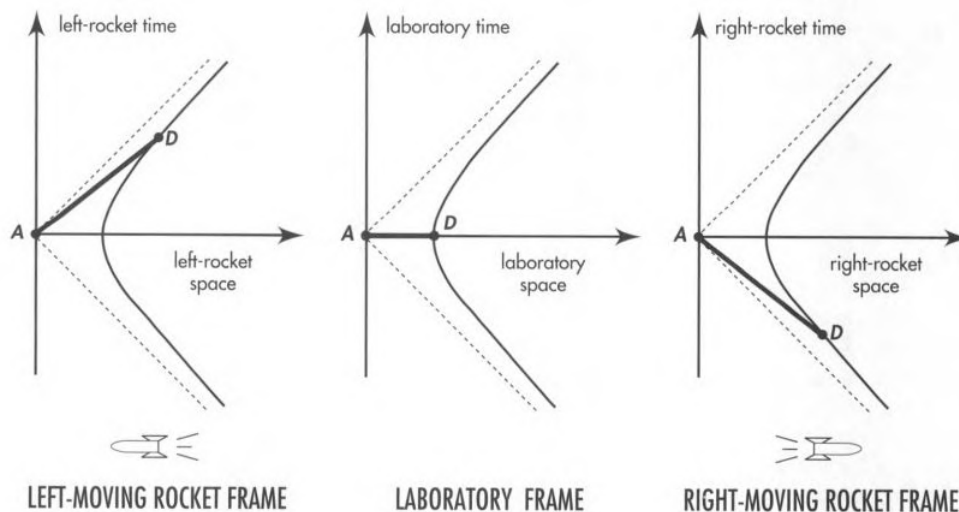
Figure 6.2.2: The spacelike pair of events A and D (with event A arbitrarily chosen as reference event) as recorded in the spacetime maps of three free-float frames. Point D lies on a hyperbola opening along the space axis in every rocket and laboratory frame. The shortest distance between these events is recorded in the laboratory frame, the frame in which the two events occur at the same time. A heavy line represents the spacetime separation AD . No particle can travel along this line; the speed would be greater than light speed—and would be infinitely great as measured in the laboratory frame, since the particle would have to cover the distance from A to D in zero time!
