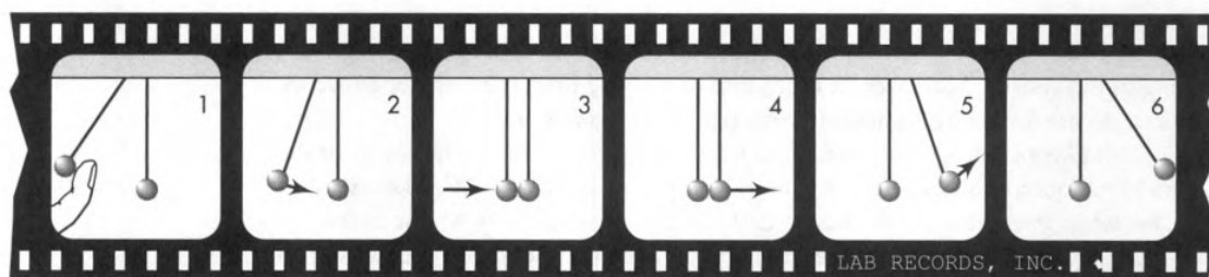
Figure 8.2.1: One marble collides elastically with another.
