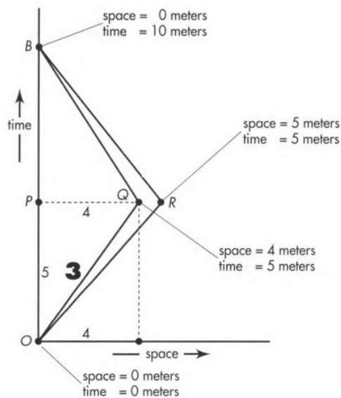
Figure 5.7.1: Three alternative worldlines connecting events O and B. The sharp changes of velocity at events Q and R have been drawn for the ideal limit of small clocks that tolerate great acceleration. The bold-face number 3 is the proper time along the segment OQ, reckoned from the difference between the squared time separation and the squared space separation: 3^2 = 5^2 - 4^2 .
