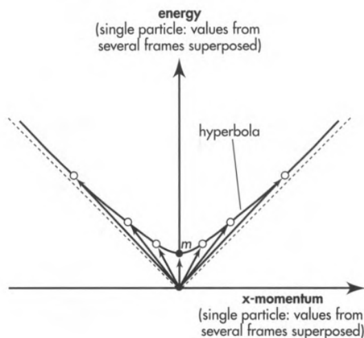
Figure 7.3.1: Momenergy 4-vector for the single particle of Figure 7 – 3 as observed in seven free-float frames, these plots then superposed on a composite momenergy diagram. Frames are chosen so that y - and z -components of momentum equal zero. Locus of the tips of the arrows traces out a hyperbola. The central short vertical arrow pointing to the dot labeled m represents momenergy as measured in the particle rest frame. In this frame momentum has value zero and energy- "rest energy"-equals the mass of the particle. For clarity, the handles have been omitted from the 4 vectors, which all have identical invariant magnitude m = 20 . consequence is that the particle moves at less than the speed of light in every possible free-float frame.
