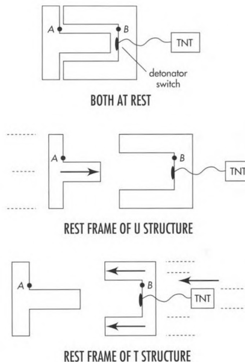
Figure 6.E.2: Both at rest: The leg of the T almost reaches the detonator switch when both the T and the U are at rest. Points A and B are used in part b of the exercise. Rest frame of U structure: The leg of the moving T is Lorentz contracted in the rest frame of the U. Does this mean that the explosion will not take place? Rest frame of T structure: The legs of the moving U are Lorentz-contracted in the rest frame of the T. Does this mean explosion will take place?
