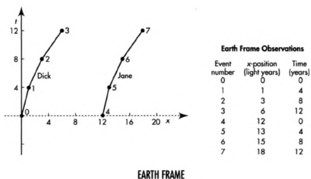
Worldlines of Dick and Jane as observed in the Earth frame of Mom and Dad.
