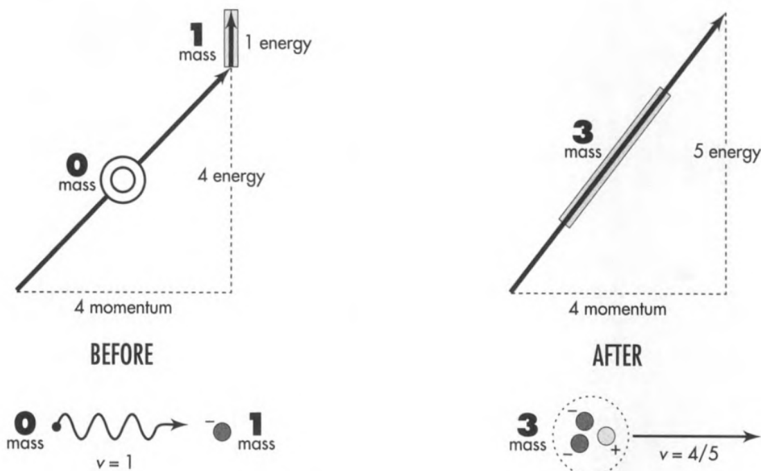
Figure 8.5.2: Conservation of energy and momentum in the process of creating a pair (a positive and a negative electron) in the field of an electron. Before: A photon that has energy (and momentum) equal to four electron masses (sloping arrow) strikes an electron essentially at rest (vertical arrow). After: The photon has ceased to exist, and the two newly created particles have gone off in company with the original electron at 80 percent of light speed—a combined “particle” of three electron masses
