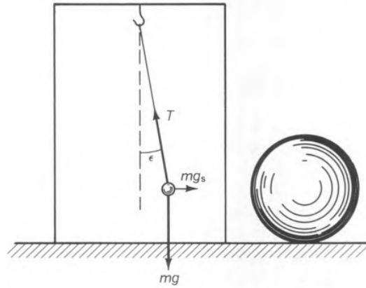
Right: Rolling the sphere to the other side results in static deflection of plumb line in the opposite direction.
