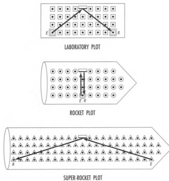
Figure 3.7.2: Plots of the path in space of a reflected flash of light as measured in three different frames, showing event E, emission of the flash, and event R, its reception after reflection. Squares, circles, and triangles represent latticeworks of recording clocks in laboratory, rocket, and super-rocket frames, respectively. The super-rocket frame moves to the right with respect to the rocket, and with such relative speed that the event of reception, R, occurs to the left of the event of emission, E, as measured in the super-rocket frame. The reflecting mirror is fixed in the rocket, hence appears to move from left to right in the laboratory and from right to left in the super-rocket.
