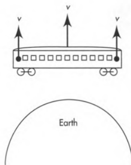
Figure 2.E.2: Free-float railway coach rising from Earth's surface, as observed in Earth frame. Two ball bearings were just released from rest with respect to the coach. What will be their subsequent motion as observed from inside the coach? Figure not to scale.
