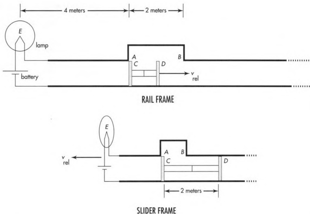
Figure 6.E.3: Rail frame: Configuration at t = 0 in the rest frame of the rails. Slider CD moves to the right with speed v_{rel} such that the Lorentz-contraction factor equals 2. The vertical legs of the slider are conductors; the horizontal crosspiece is an insulator. Slider frame: Configuration at t' = 0 in the rest frame of the slider. The rails and lamp move to the left with speed v_{rel} such that the Lorentz-contraction factor is 2.
