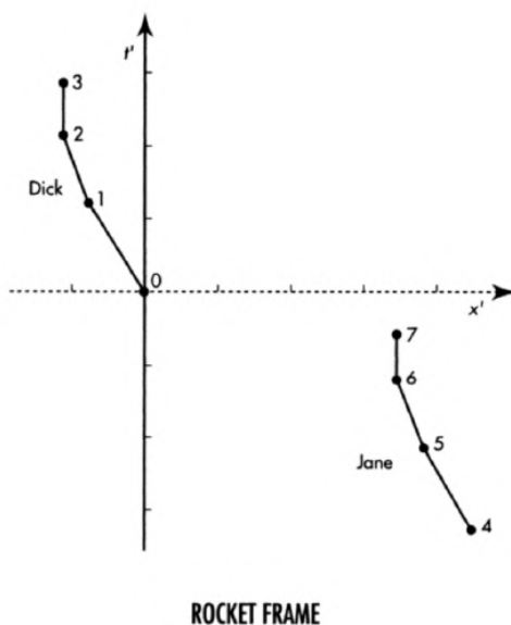
Worldlines of Dick and Jane as observed in the "final" rocket frame in which both Dick and Jane come to rest after burnout.
