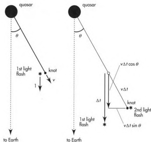
Figure 3.E.11: first figure. Left: Bright "knot" of plasma ejected from a quasar at high speed v emits a first flash of light toward Earth. Right: The knot emits a second light flash toward Earth a time \Delta t later. This time \Delta t is measured locally near the knot using the Earth-linked latticework of rods and clocks (bar! bar!).
