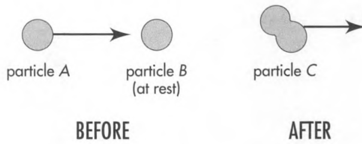
Figure 7.E.3: Two putty balls stick together
