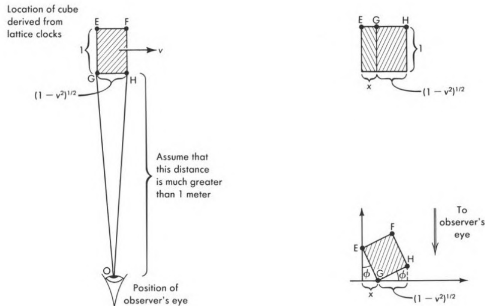
Figure 3.E.13: Left: Position of eye of visual observer watching cube pass overhead. Right top: What the visual observer sees as she looks up from below. Right bottom: How the visual observer can interpret the projection of the second figure.
