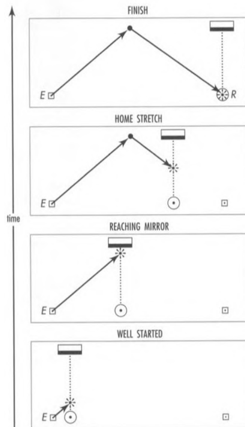
Figure 3.7.1: Plot of the flash path as recorded in the laboratory frame. Time progresses from bottom to top: Well started: The flash (represented as an asterisk) has been emitted (event E) from a moving rocket clock (shown as a circle) that coincided with a laboratory clock (shown as a square). Reaching mirror and Home stretch: The flash reaches a mirror and reflects from it. The mirror moves along in step with the rocket clock. Finish: The flash is received (event R) back at the same rocket clock, which has moved in the laboratory frame to coincide with a second laboratory clock. Figure 3.7.2 shows the trajectory of the same flash in three different free-float frames.
