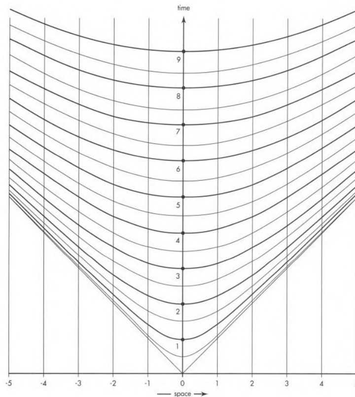
Figure 5.E.3: Template of hyperbolas you can lay it over the hyperbola on thin paper so you can lay it over the hyperbola graph and see the hyperbolas.
