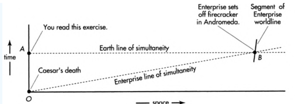
Figure 11.7.1: Earth spacetime diagram, showing events O , A , and B . Not to scale.
