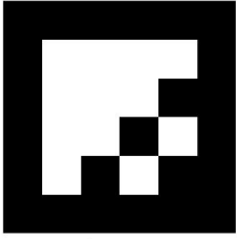
♟ WP1 ID: 8
