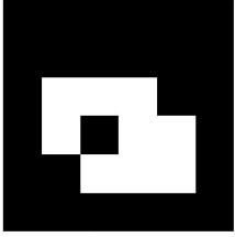
♞ WP5 ID: 12
