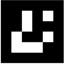
♘ WB1 ID: 4
