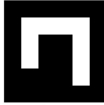
♝ WP3 ID: 10
