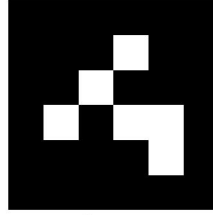
♟ WP7 ID: 14
