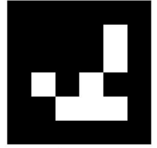
♞ WP4 ID: 11
