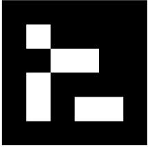
♞ BB1 ID: 20
