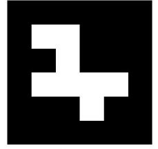
♟ WN2 ID: 7
