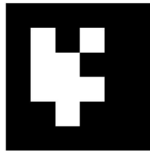
♞ BP3 ID: 26
