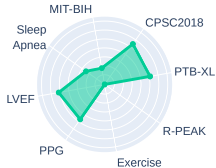
ECG Founder
