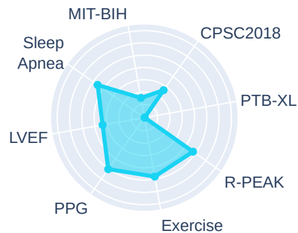
supervised(xlstm)
