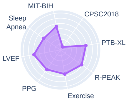
ours (transformer)
